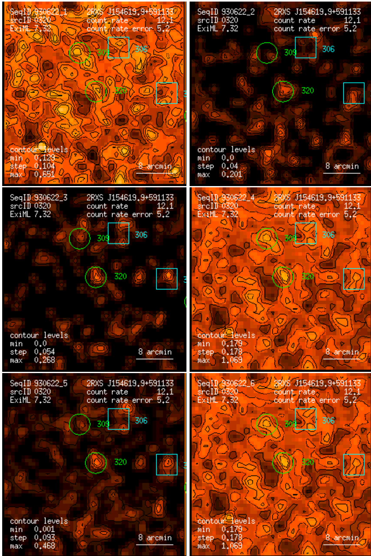
Figure 320: RASS 930622: detection 0320: band rate images, Gaussian filter: (1) PSPC channels 11 – 41, (2) 52 – 90, (3) 91 – 201, (4) 11 – 235, (5) 52 – 201, (6) 11 – 201. Broad band rates in counts/ks. Band rate contour levels in counts/ks/arcmin 2 .
