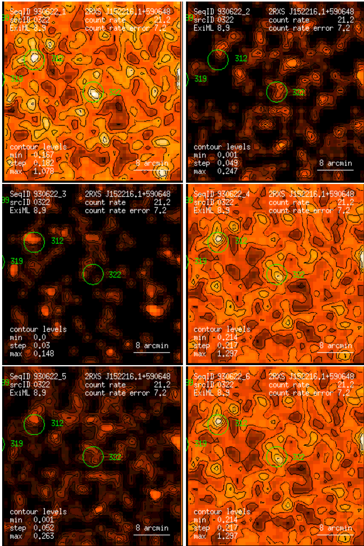
Figure 322: RASS 930622: detection 0322: band rate images, Gaussian filter: (1) PSPC channels 11 – 41, (2) 52 – 90, (3) 91 – 201, (4) 11 – 235, (5) 52 – 201, (6) 11 – 201. Broad band rates in counts/ks. Band rate contour levels in counts/ks/arcmin 2 .
