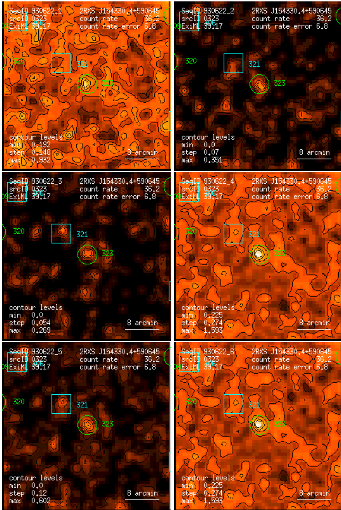
Figure 323: RASS 930622: detection 0323: band rate images, Gaussian filter: (1) PSPC channels 11 – 41, (2) 52 – 90, (3) 91 – 201, (4) 11 – 235, (5) 52 – 201, (6) 11 – 201. Broad band rates in counts/ks. Band rate contour levels in counts/ks/arcmin 2 .
