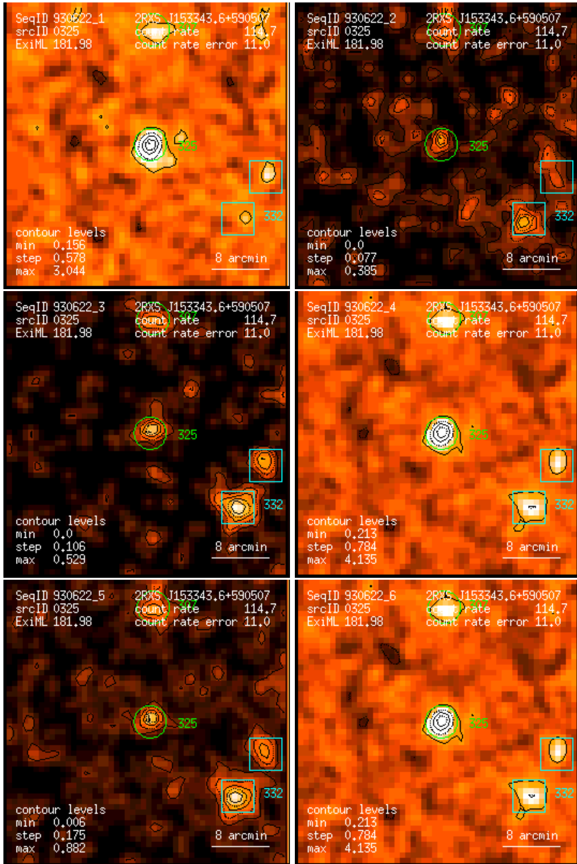
Figure 325: RASS 930622: detection 0325: band rate images, Gaussian filter: (1) PSPC channels 11 – 41, (2) 52 – 90, (3) 91 – 201, (4) 11 – 235, (5) 52 – 201, (6) 11 – 201. Broad band rates in counts/ks. Band rate contour levels in counts/ks/arcmin 2 .
