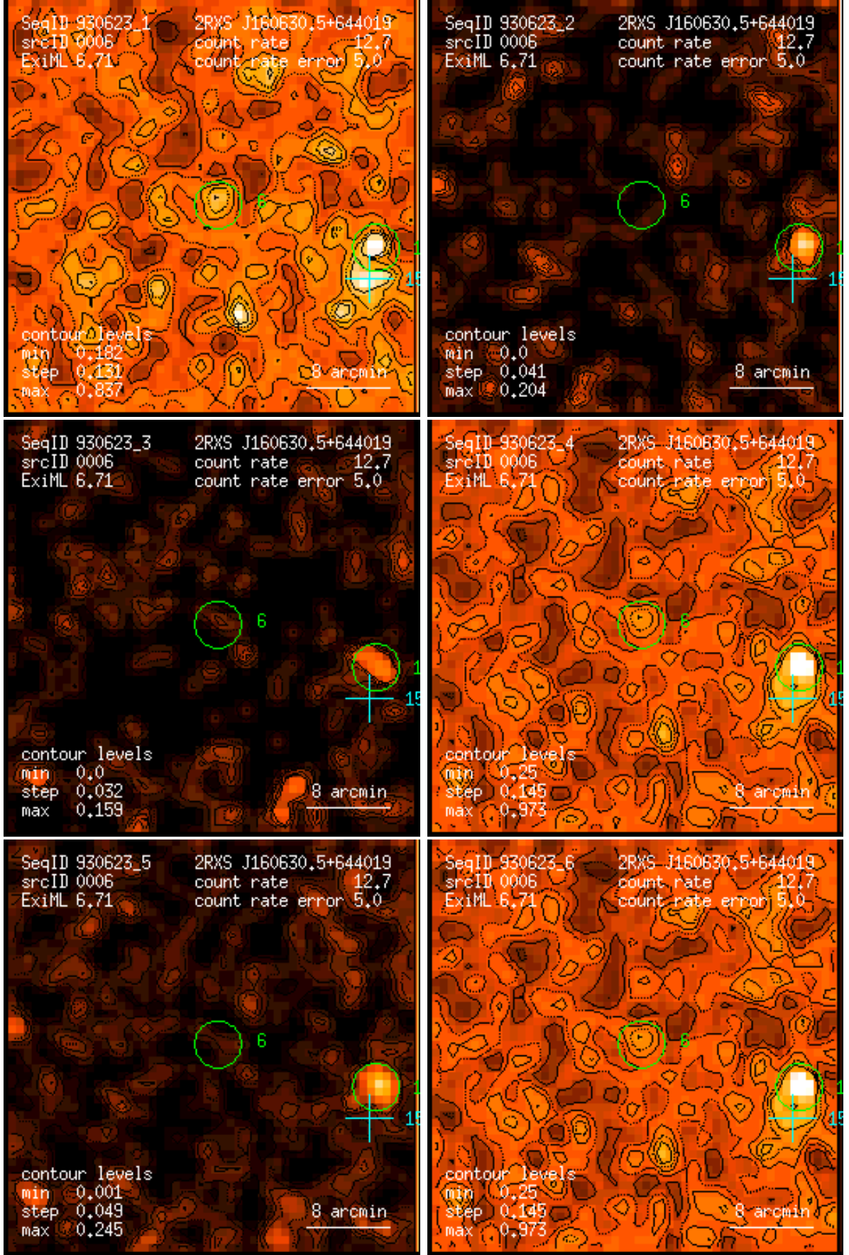
Figure 6: RASS 930623: detection 0006: band rate images, Gaussian filter: (1) PSPC channels 11 – 41, (2) 52 – 90, (3) 91 – 201, (4) 11 – 235, (5) 52 – 201, (6) 11 – 201. Broad band rates in counts/ks. Band rate contour levels in counts/ks/arcmin 2 .
