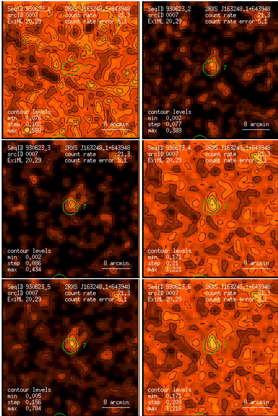
Figure 7: RASS 930623: detection 0007: band rate images, Gaussian filter: (1) PSPC channels 11 – 41, (2) 52 – 90, (3) 91 – 201, (4) 11 – 235, (5) 52 – 201, (6) 11 – 201. Broad band rates in counts/ks. Band rate contour levels in counts/ks/arcmin 2 .
