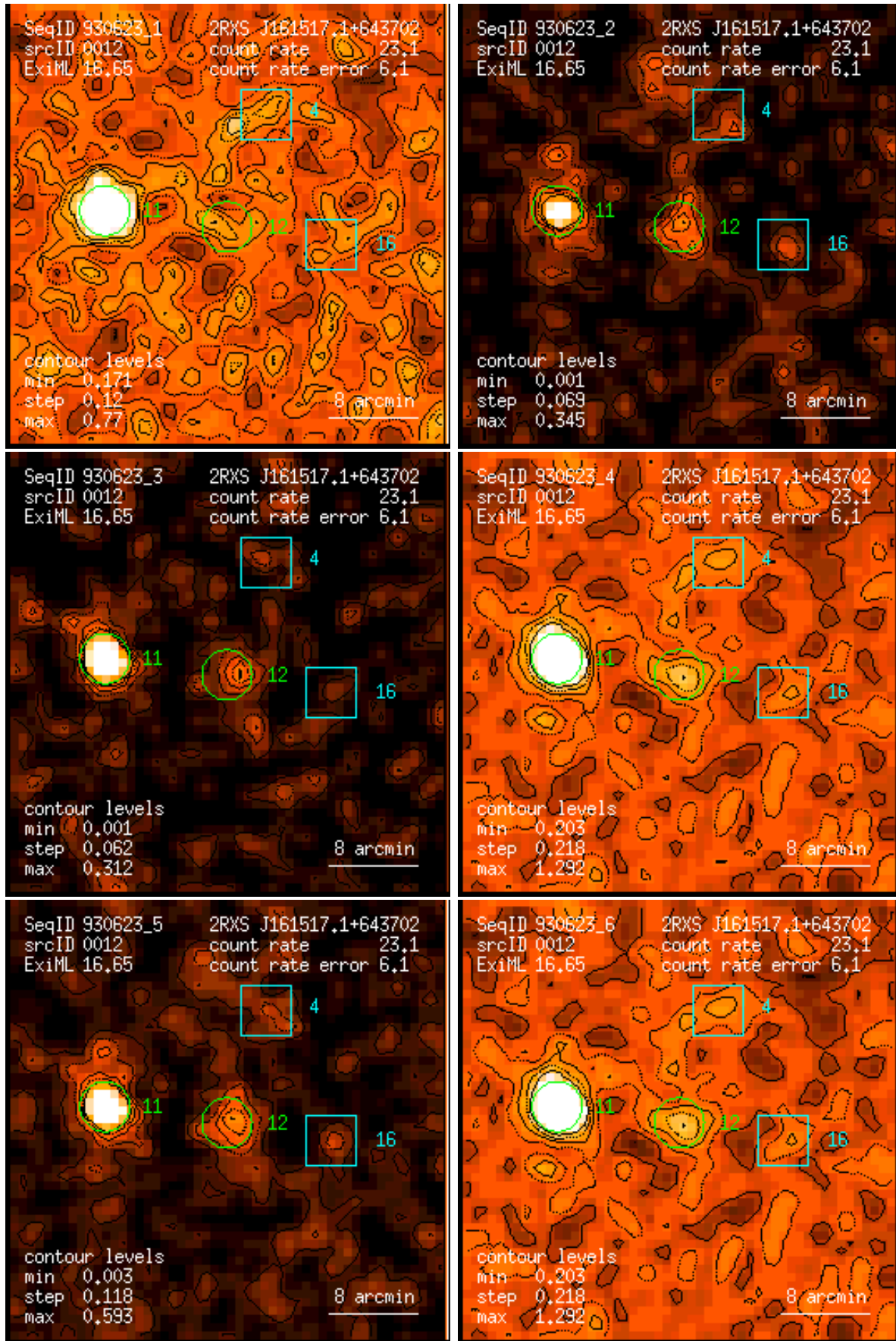
Figure 12: RASS 930623: detection 0012: band rate images, Gaussian filter: (1) PSPC channels 11 – 41, (2) 52 – 90, (3) 91 – 201, (4) 11 – 235, (5) 52 – 201, (6) 11 – 201. Broad band rates in counts/ks. Band rate contour levels in counts/ks/arcmin 2 .
