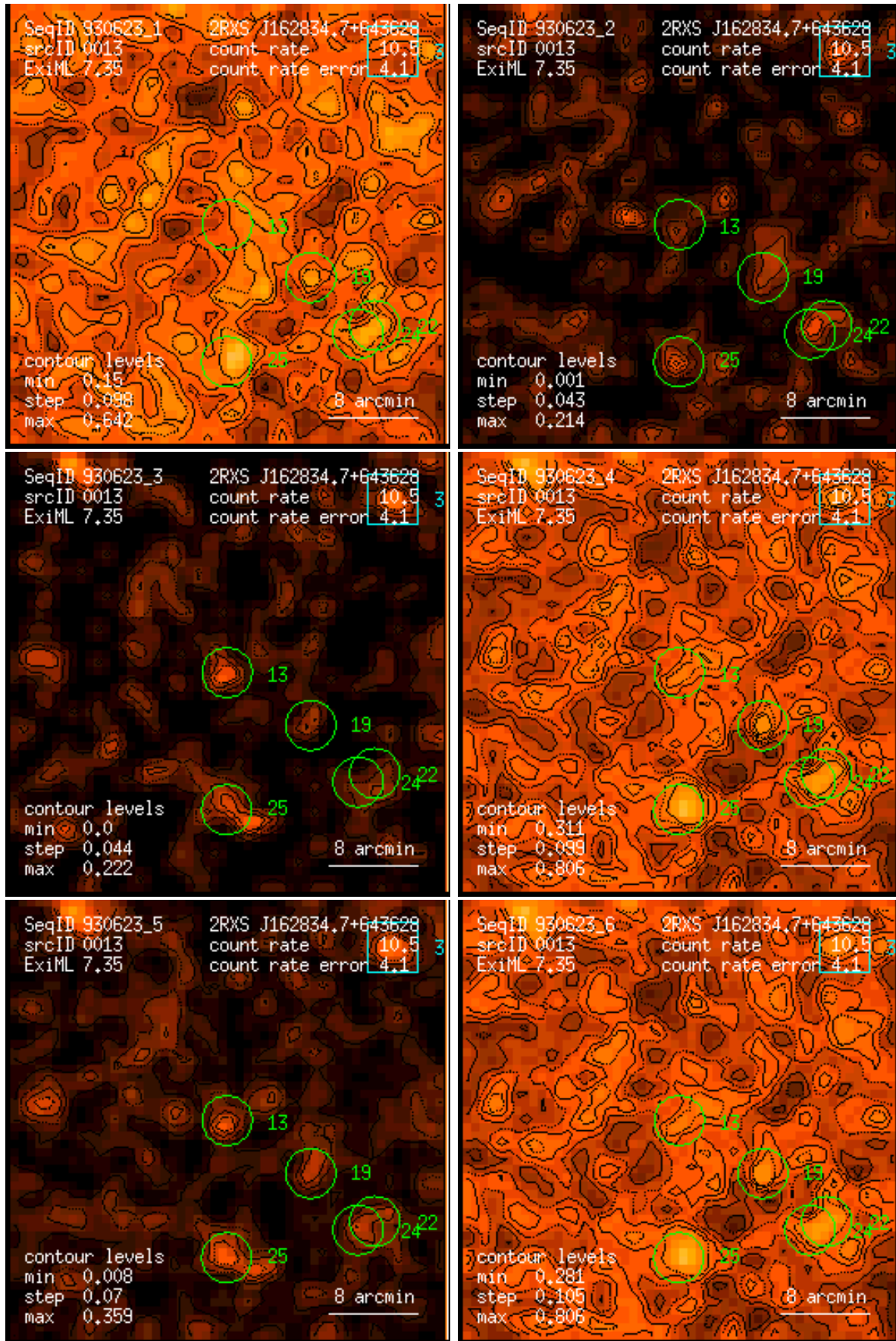
Figure 13: RASS 930623: detection 0013: band rate images, Gaussian filter: (1) PSPC channels 11 – 41, (2) 52 – 90, (3) 91 – 201, (4) 11 – 235, (5) 52 – 201, (6) 11 – 201. Broad band rates in counts/ks. Band rate contour levels in counts/ks/arcmin 2 .
