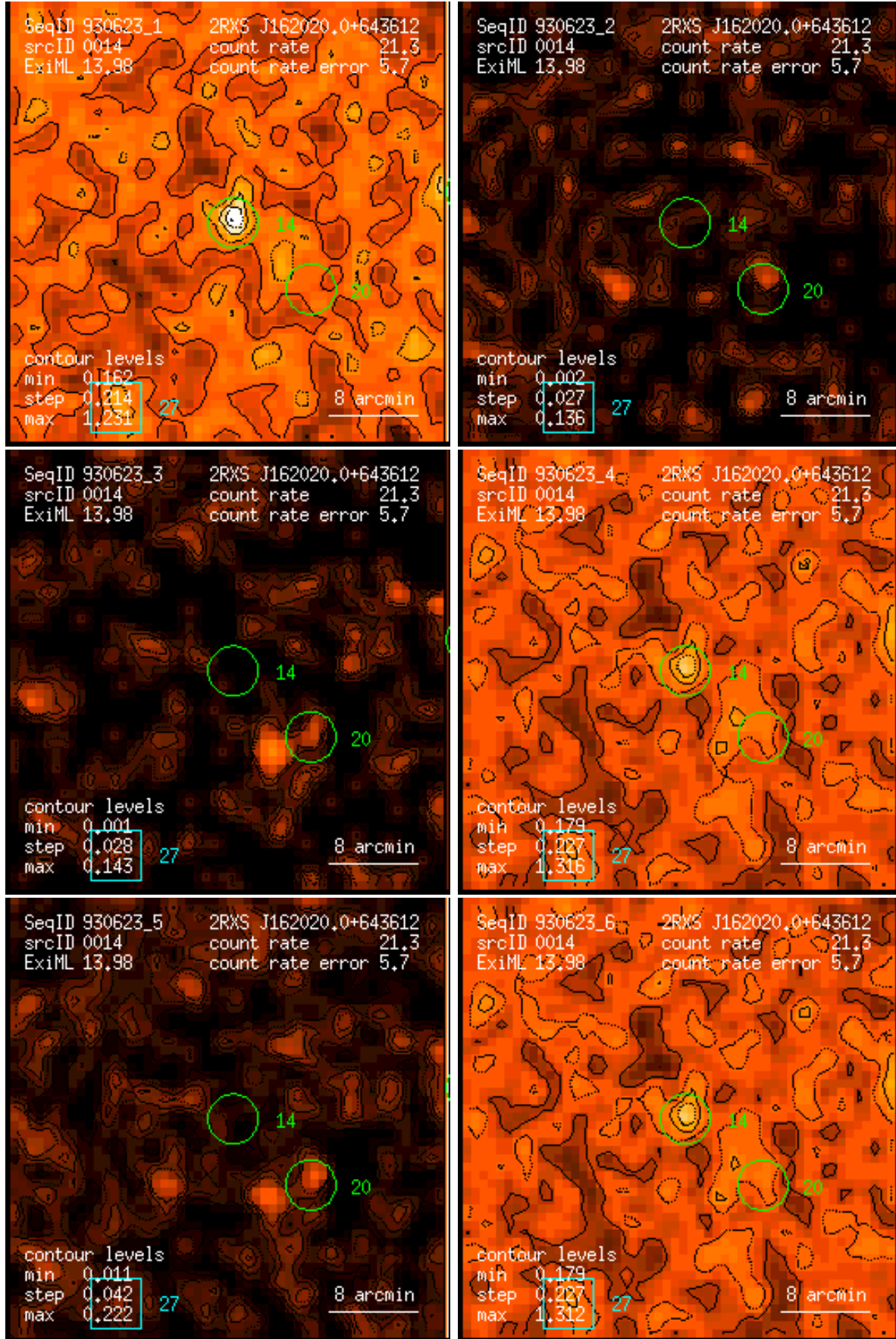
Figure 14: RASS 930623: detection 0014: band rate images, Gaussian filter: (1) PSPC channels 11 – 41, (2) 52 – 90, (3) 91 – 201, (4) 11 – 235, (5) 52 – 201, (6) 11 – 201. Broad band rates in counts/ks. Band rate contour levels in counts/ks/arcmin 2 .
