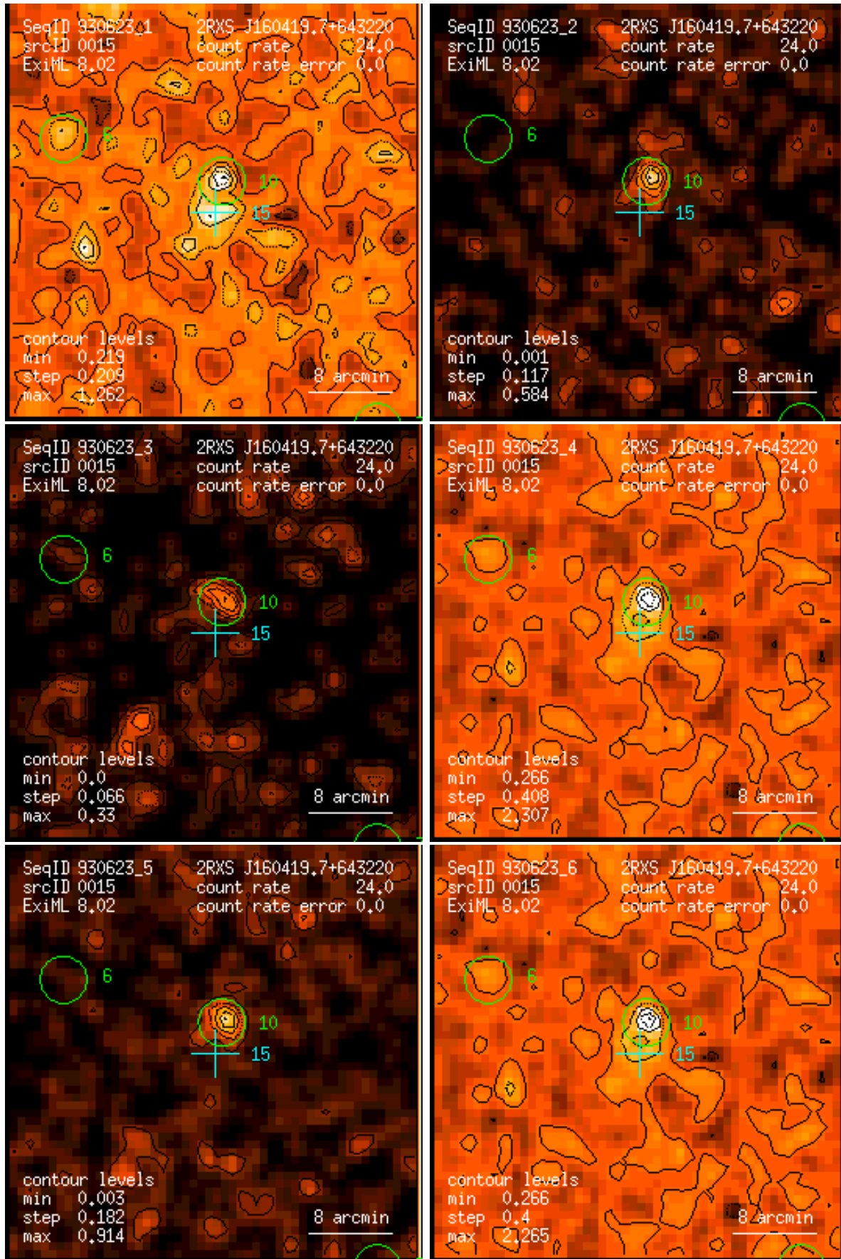
Figure 15: RASS 930623: detection 0015: band rate images, Gaussian filter: (1) PSPC channels 11 – 41, (2) 52 – 90, (3) 91 – 201, (4) 11 – 235, (5) 52 – 201, (6) 11 – 201. Broad band rates in counts/ks. Band rate contour levels in counts/ks/arcmin 2 .
