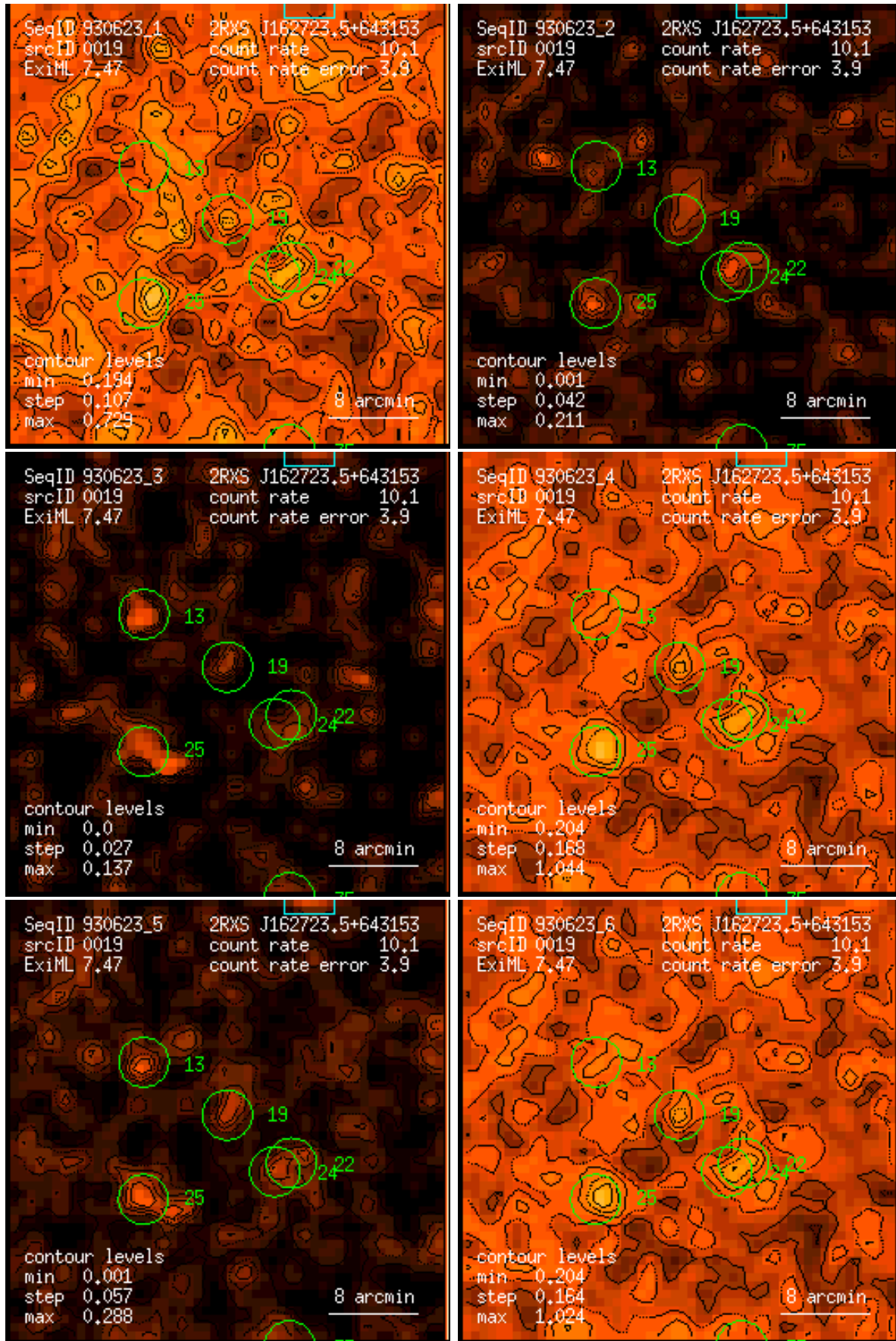
Figure 19: RASS 930623: detection 0019: band rate images, Gaussian filter: (1) PSPC channels 11 – 41, (2) 52 – 90, (3) 91 – 201, (4) 11 – 235, (5) 52 – 201, (6) 11 – 201. Broad band rates in counts/ks. Band rate contour levels in counts/ks/arcmin 2 .
