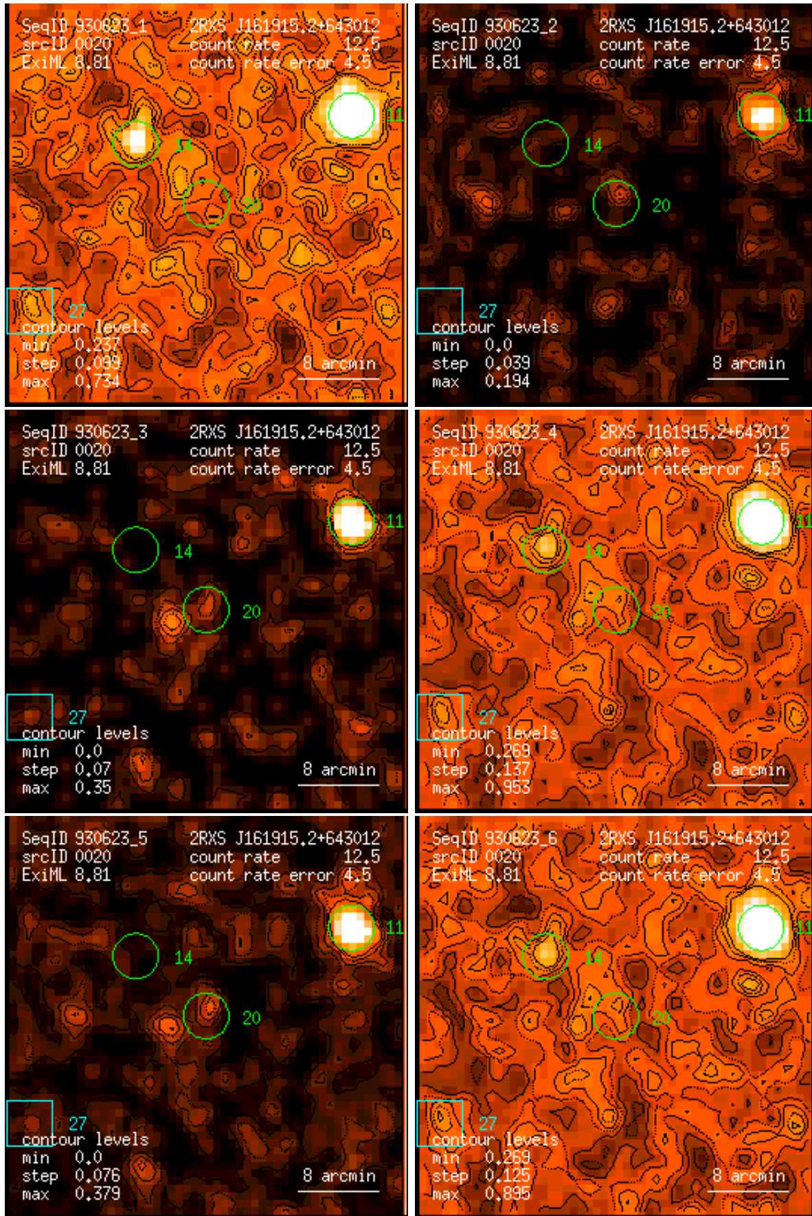
Figure 20: RASS 930623: detection 0020: band rate images, Gaussian filter: (1) PSPC channels 11 – 41, (2) 52 – 90, (3) 91 – 201, (4) 11 – 235, (5) 52 – 201, (6) 11 – 201. Broad band rates in counts/ks. Band rate contour levels in counts/ks/arcmin 2 .
