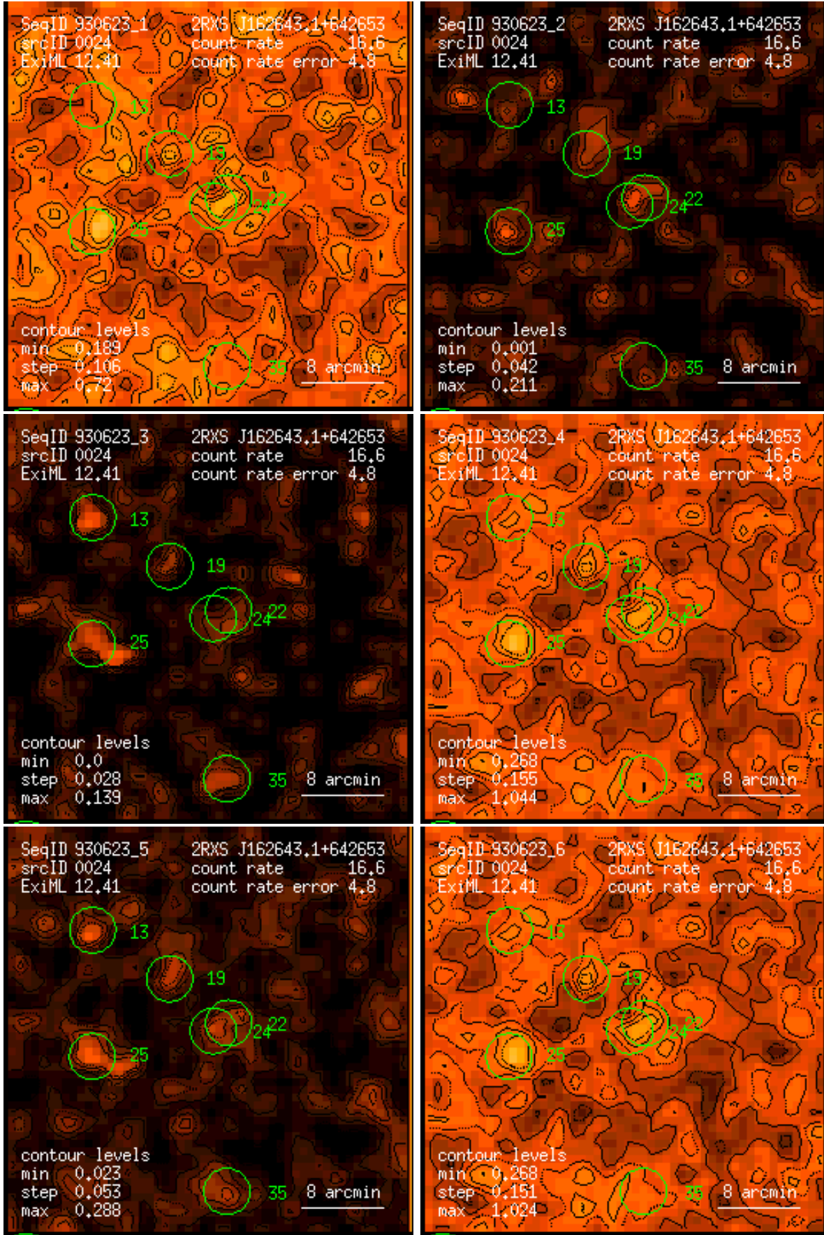
Figure 24: RASS 930623: detection 0024: band rate images, Gaussian filter: (1) PSPC channels 11 – 41, (2) 52 – 90, (3) 91 – 201, (4) 11 – 235, (5) 52 – 201, (6) 11 – 201. Broad band rates in counts/ks. Band rate contour levels in counts/ks/arcmin 2 .
