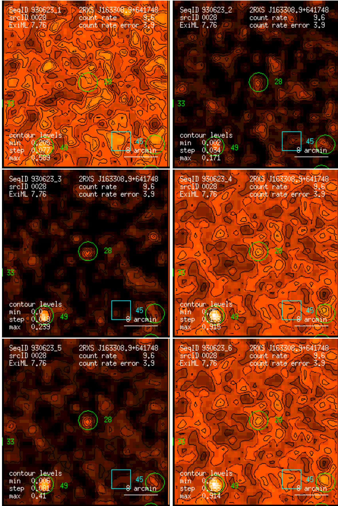
Figure 28: RASS 930623: detection 0028: band rate images, Gaussian filter: (1) PSPC channels 11 – 41, (2) 52 – 90, (3) 91 – 201, (4) 11 – 235, (5) 52 – 201, (6) 11 – 201. Broad band rates in counts/ks. Band rate contour levels in counts/ks/arcmin 2 .
