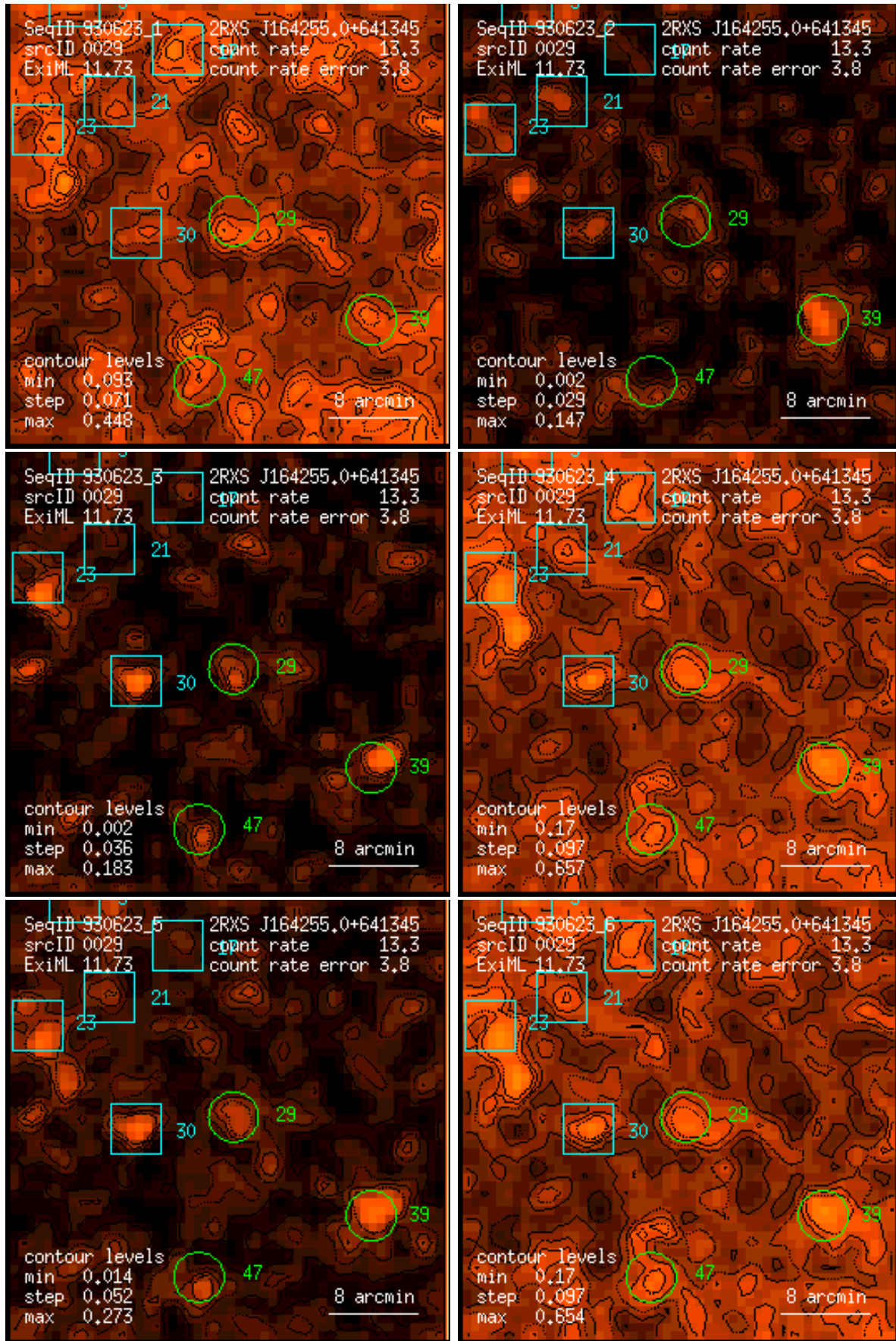
Figure 29: RASS 930623: detection 0029: band rate images, Gaussian filter: (1) PSPC channels 11 – 41, (2) 52 – 90, (3) 91 – 201, (4) 11 – 235, (5) 52 – 201, (6) 11 – 201. Broad band rates in counts/ks. Band rate contour levels in counts/ks/arcmin 2 .
