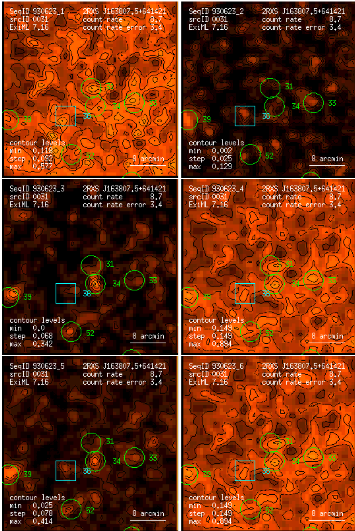
Figure 31: RASS 930623: detection 0031: band rate images, Gaussian filter: (1) PSPC channels 11 – 41, (2) 52 – 90, (3) 91 – 201, (4) 11 – 235, (5) 52 – 201, (6) 11 – 201. Broad band rates in counts/ks. Band rate contour levels in counts/ks/arcmin 2 .
