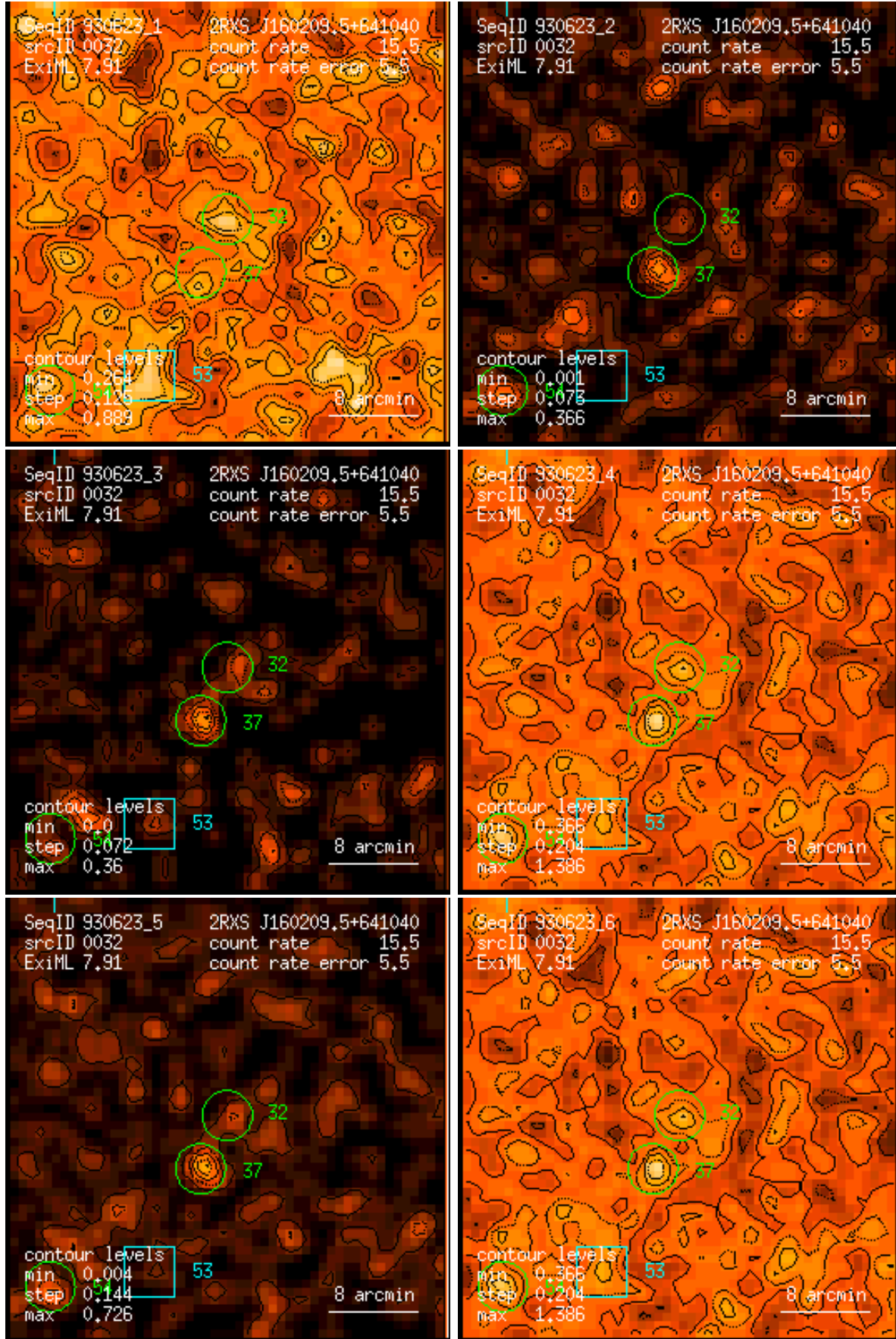
Figure 32: RASS 930623: detection 0032: band rate images, Gaussian filter: (1) PSPC channels 11 – 41, (2) 52 – 90, (3) 91 – 201, (4) 11 – 235, (5) 52 – 201, (6) 11 – 201. Broad band rates in counts/ks. Band rate contour levels in counts/ks/arcmin 2 .
