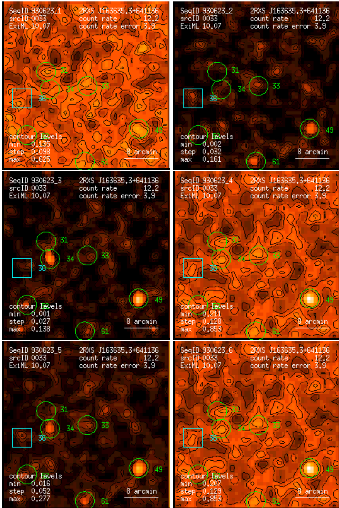
Figure 33: RASS 930623: detection 0033: band rate images, Gaussian filter: (1) PSPC channels 11 – 41, (2) 52 – 90, (3) 91 – 201, (4) 11 – 235, (5) 52 – 201, (6) 11 – 201. Broad band rates in counts/ks. Band rate contour levels in counts/ks/arcmin 2 .
