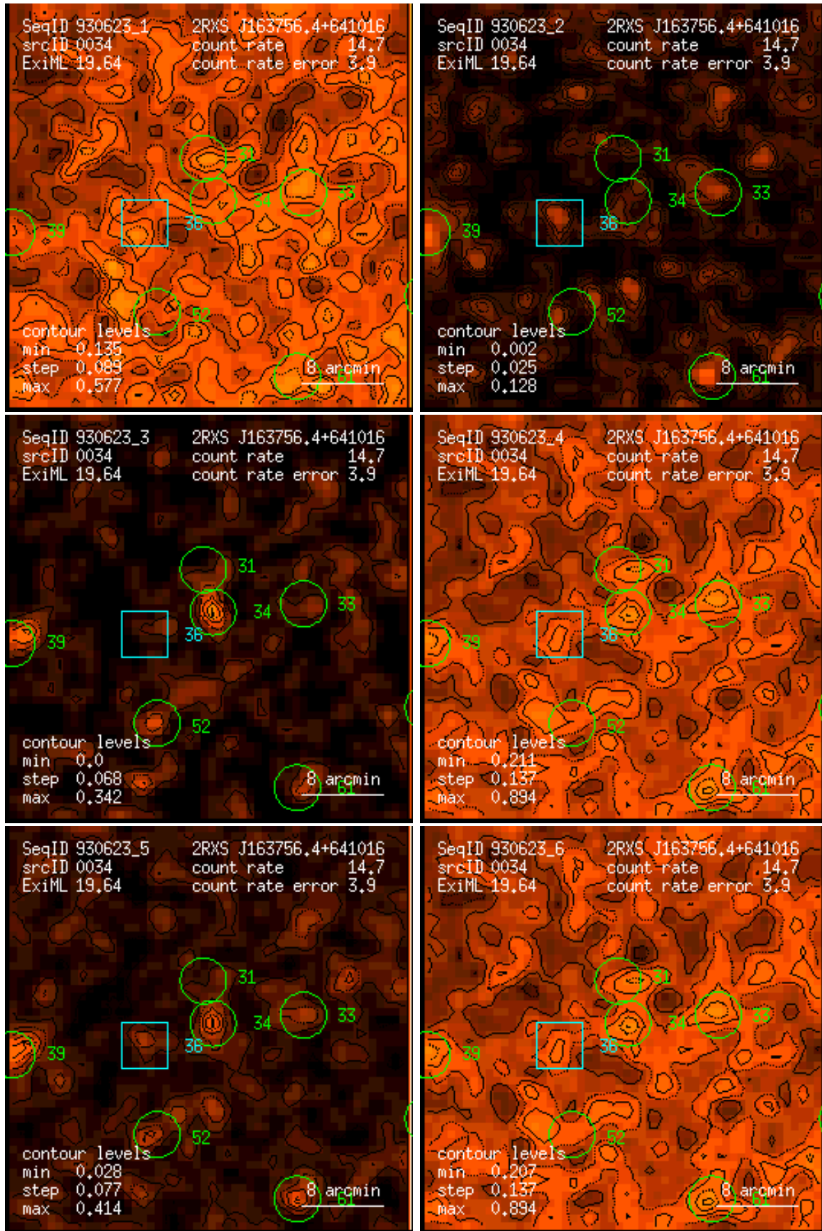
Figure 34: RASS 930623: detection 0034: band rate images, Gaussian filter: (1) PSPC channels 11 – 41, (2) 52 – 90, (3) 91 – 201, (4) 11 – 235, (5) 52 – 201, (6) 11 – 201. Broad band rates in counts/ks. Band rate contour levels in counts/ks/arcmin 2 .
