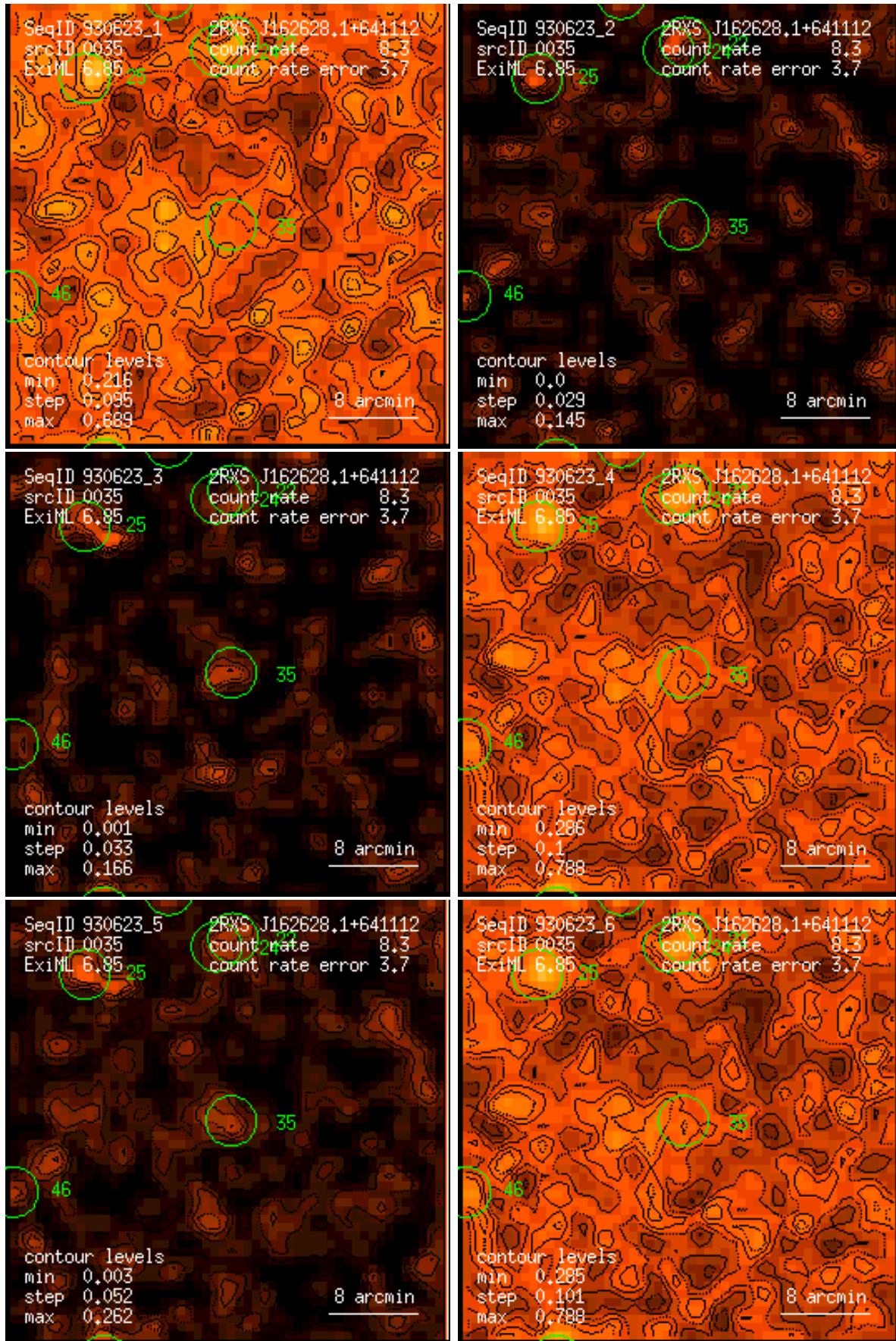
Figure 35: RASS 930623: detection 0035: band rate images, Gaussian filter: (1) PSPC channels 11 – 41, (2) 52 – 90, (3) 91 – 201, (4) 11 – 235, (5) 52 – 201, (6) 11 – 201. Broad band rates in counts/ks. Band rate contour levels in counts/ks/arcmin 2 .
