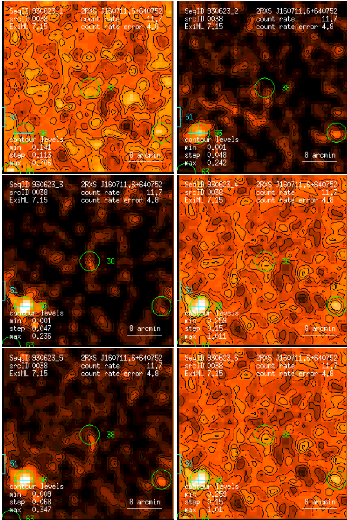
Figure 38: RASS 930623: detection 0038: band rate images, Gaussian filter: (1) PSPC channels 11 – 41, (2) 52 – 90, (3) 91 – 201, (4) 11 – 235, (5) 52 – 201, (6) 11 – 201. Broad band rates in counts/ks. Band rate contour levels in counts/ks/arcmin 2 .
