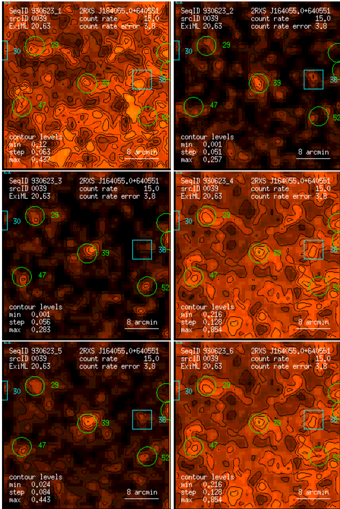
Figure 39: RASS 930623: detection 0039: band rate images, Gaussian filter: (1) PSPC channels 11 – 41, (2) 52 – 90, (3) 91 – 201, (4) 11 – 235, (5) 52 – 201, (6) 11 – 201. Broad band rates in counts/ks. Band rate contour levels in counts/ks/arcmin 2 .
