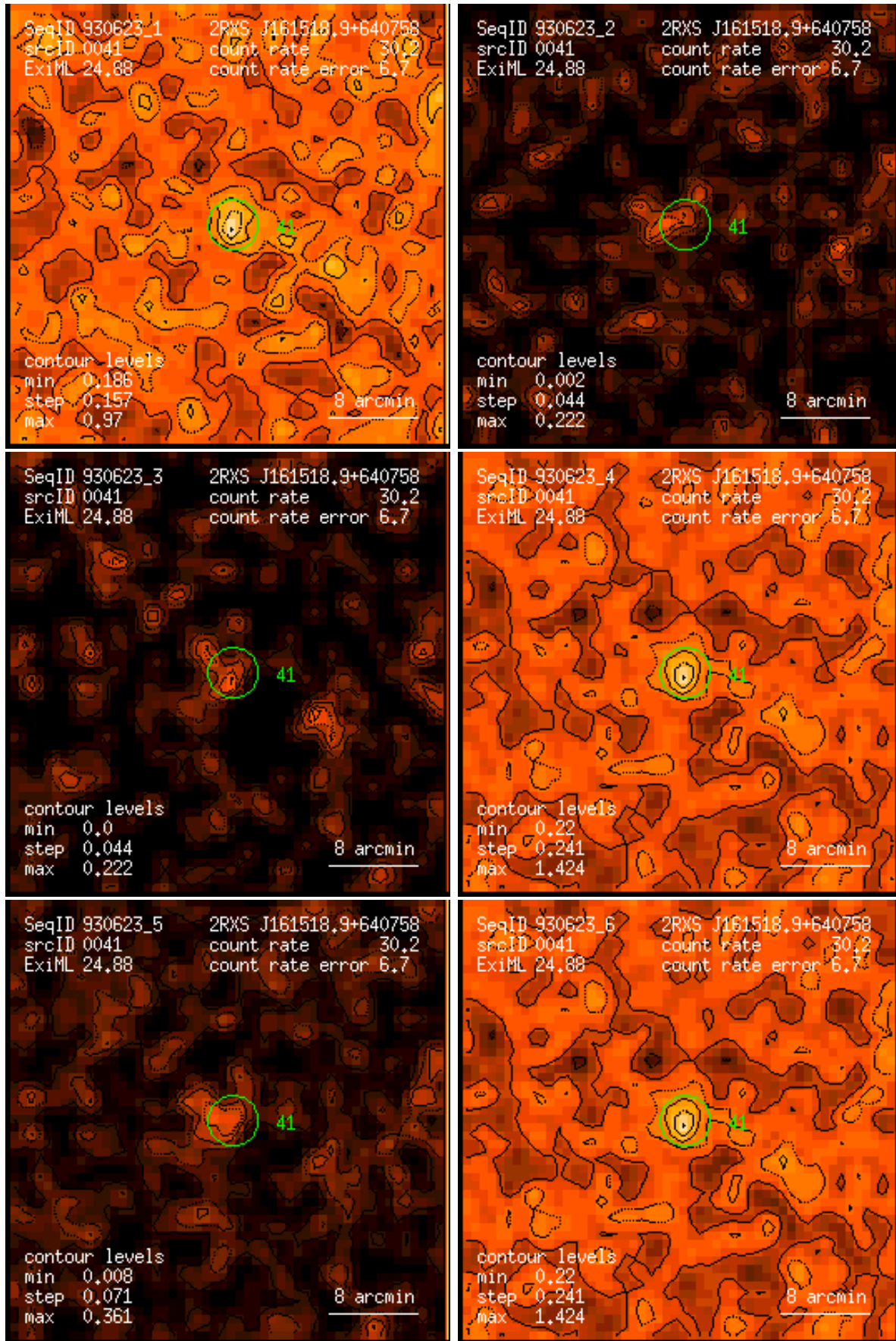
Figure 41: RASS 930623: detection 0041: band rate images, Gaussian filter: (1) PSPC channels 11 – 41, (2) 52 – 90, (3) 91 – 201, (4) 11 – 235, (5) 52 – 201, (6) 11 – 201. Broad band rates in counts/ks. Band rate contour levels in counts/ks/arcmin 2 .
