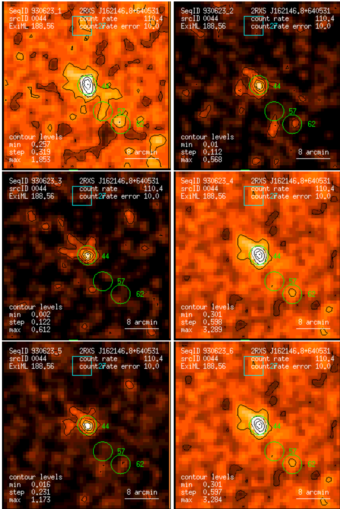
Figure 44: RASS 930623: detection 0044: band rate images, Gaussian filter: (1) PSPC channels 11 – 41, (2) 52 – 90, (3) 91 – 201, (4) 11 – 235, (5) 52 – 201, (6) 11 – 201. Broad band rates in counts/ks. Band rate contour levels in counts/ks/arcmin 2 .
