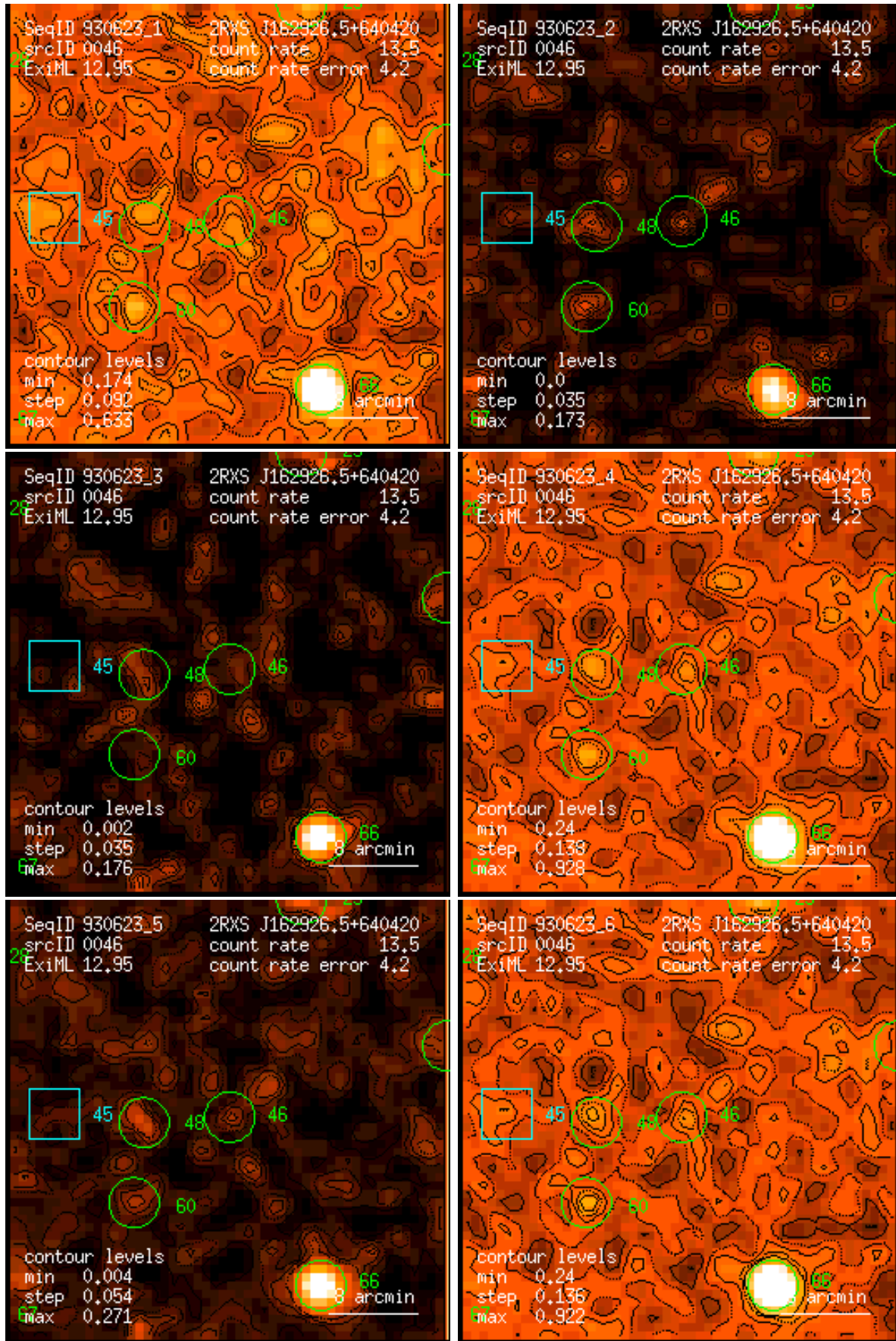
Figure 46: RASS 930623: detection 0046: band rate images, Gaussian filter: (1) PSPC channels 11 – 41, (2) 52 – 90, (3) 91 – 201, (4) 11 – 235, (5) 52 – 201, (6) 11 – 201. Broad band rates in counts/ks. Band rate contour levels in counts/ks/arcmin 2 .
