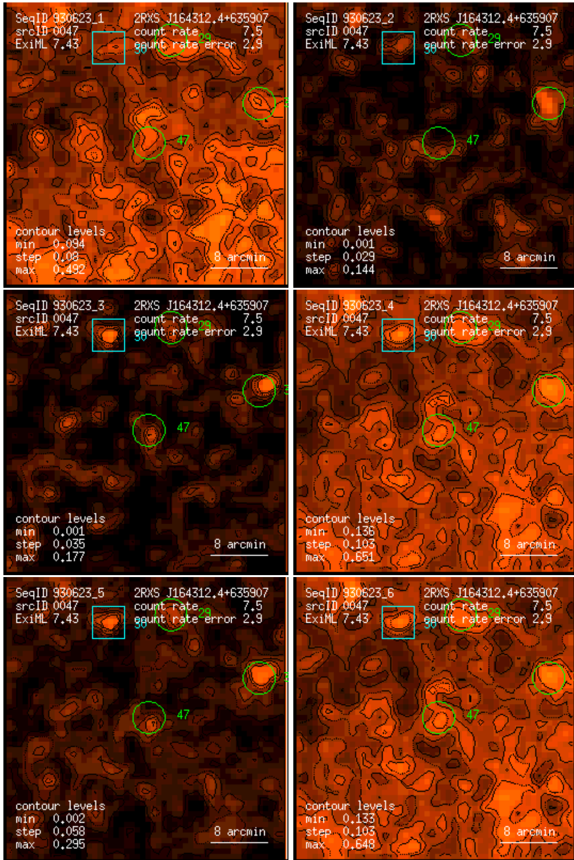
Figure 47: RASS 930623: detection 0047: band rate images, Gaussian filter: (1) PSPC channels 11 – 41, (2) 52 – 90, (3) 91 – 201, (4) 11 – 235, (5) 52 – 201, (6) 11 – 201. Broad band rates in counts/ks. Band rate contour levels in counts/ks/arcmin 2 .
