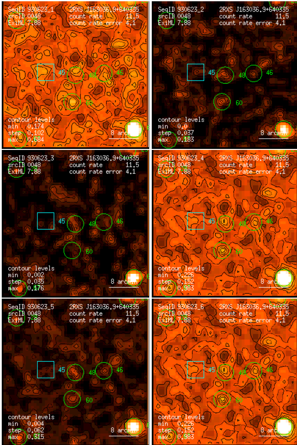
Figure 48: RASS 930623: detection 0048: band rate images, Gaussian filter: (1) PSPC channels 11 – 41, (2) 52 – 90, (3) 91 – 201, (4) 11 – 235, (5) 52 – 201, (6) 11 – 201. Broad band rates in counts/ks. Band rate contour levels in counts/ks/arcmin 2 .
