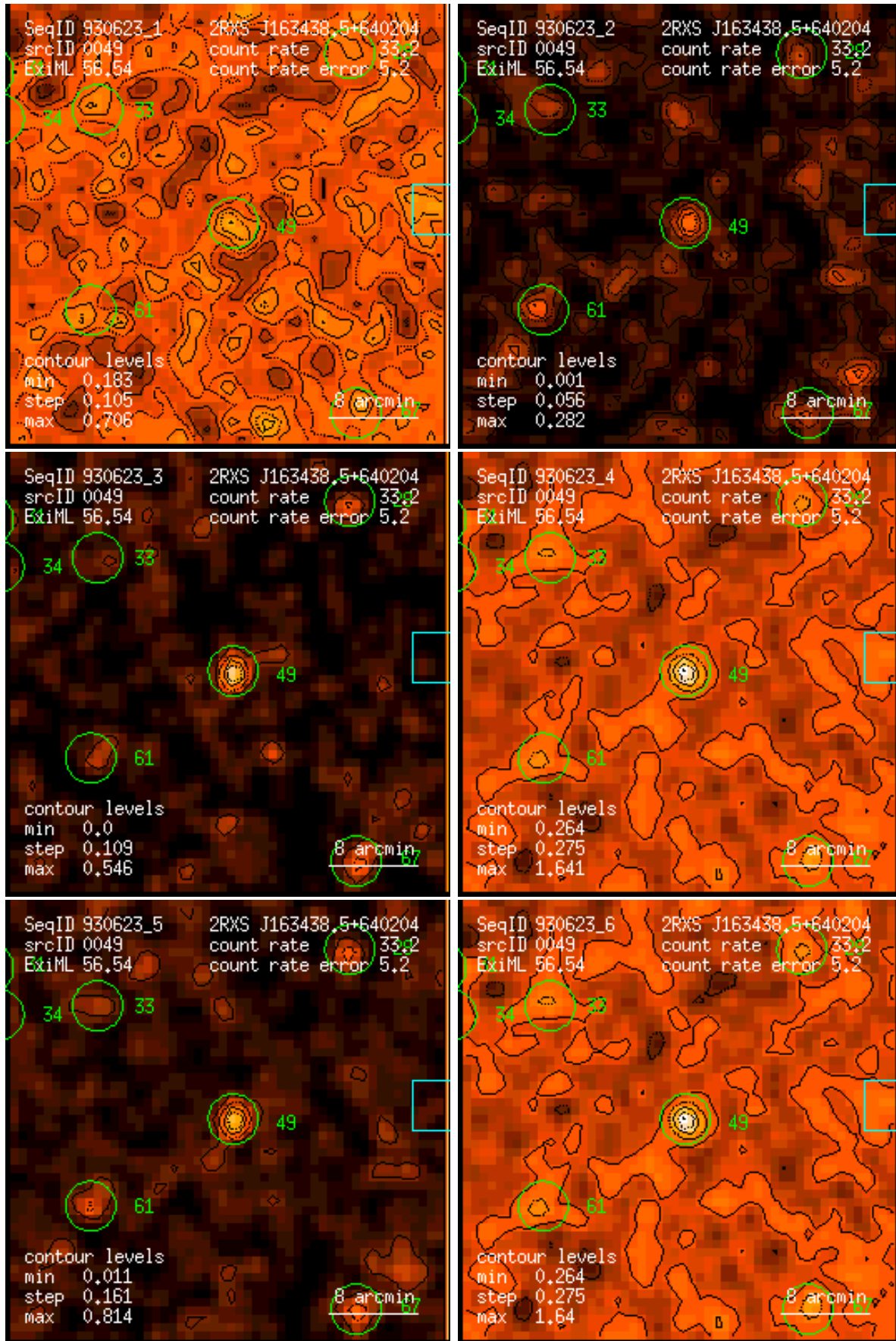
Figure 49: RASS 930623: detection 0049: band rate images, Gaussian filter: (1) PSPC channels 11 – 41, (2) 52 – 90, (3) 91 – 201, (4) 11 – 235, (5) 52 – 201, (6) 11 – 201. Broad band rates in counts/ks. Band rate contour levels in counts/ks/arcmin 2 .
