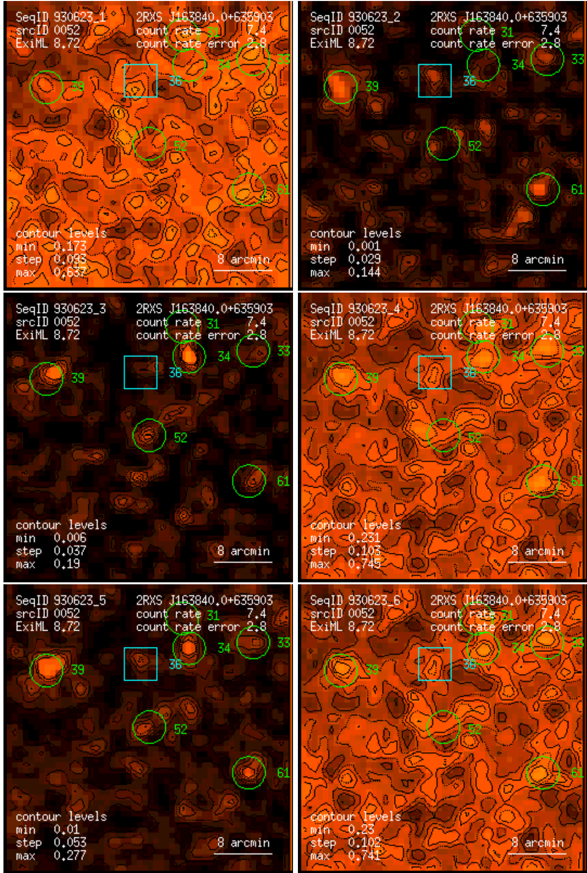
Figure 52: RASS 930623: detection 0052: band rate images, Gaussian filter: (1) PSPC channels 11 – 41, (2) 52 – 90, (3) 91 – 201, (4) 11 – 235, (5) 52 – 201, (6) 11 – 201. Broad band rates in counts/ks. Band rate contour levels in counts/ks/arcmin 2 .
