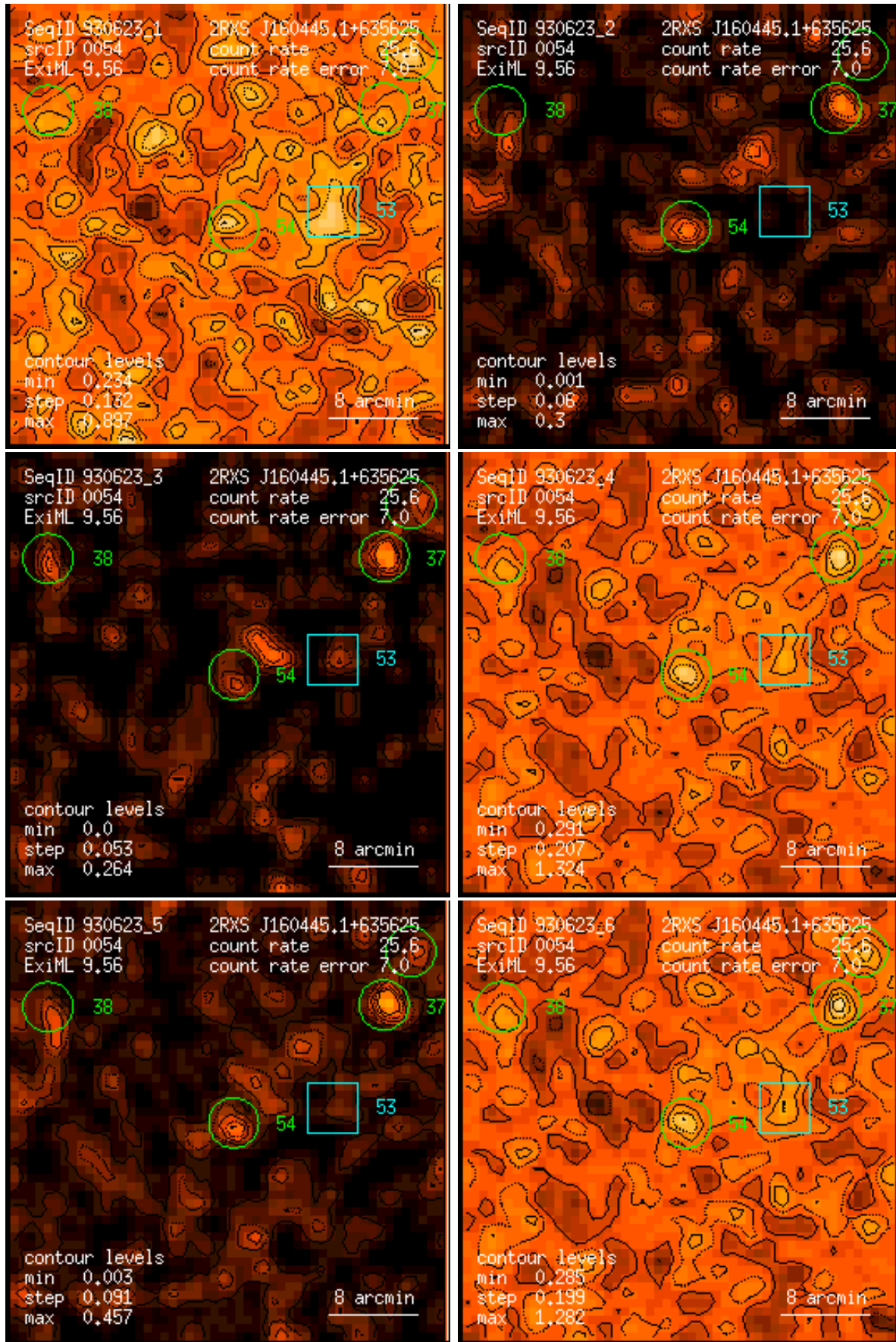
Figure 54: RASS 930623: detection 0054: band rate images, Gaussian filter: (1) PSPC channels 11 – 41, (2) 52 – 90, (3) 91 – 201, (4) 11 – 235, (5) 52 – 201, (6) 11 – 201. Broad band rates in counts/ks. Band rate contour levels in counts/ks/arcmin 2 .
