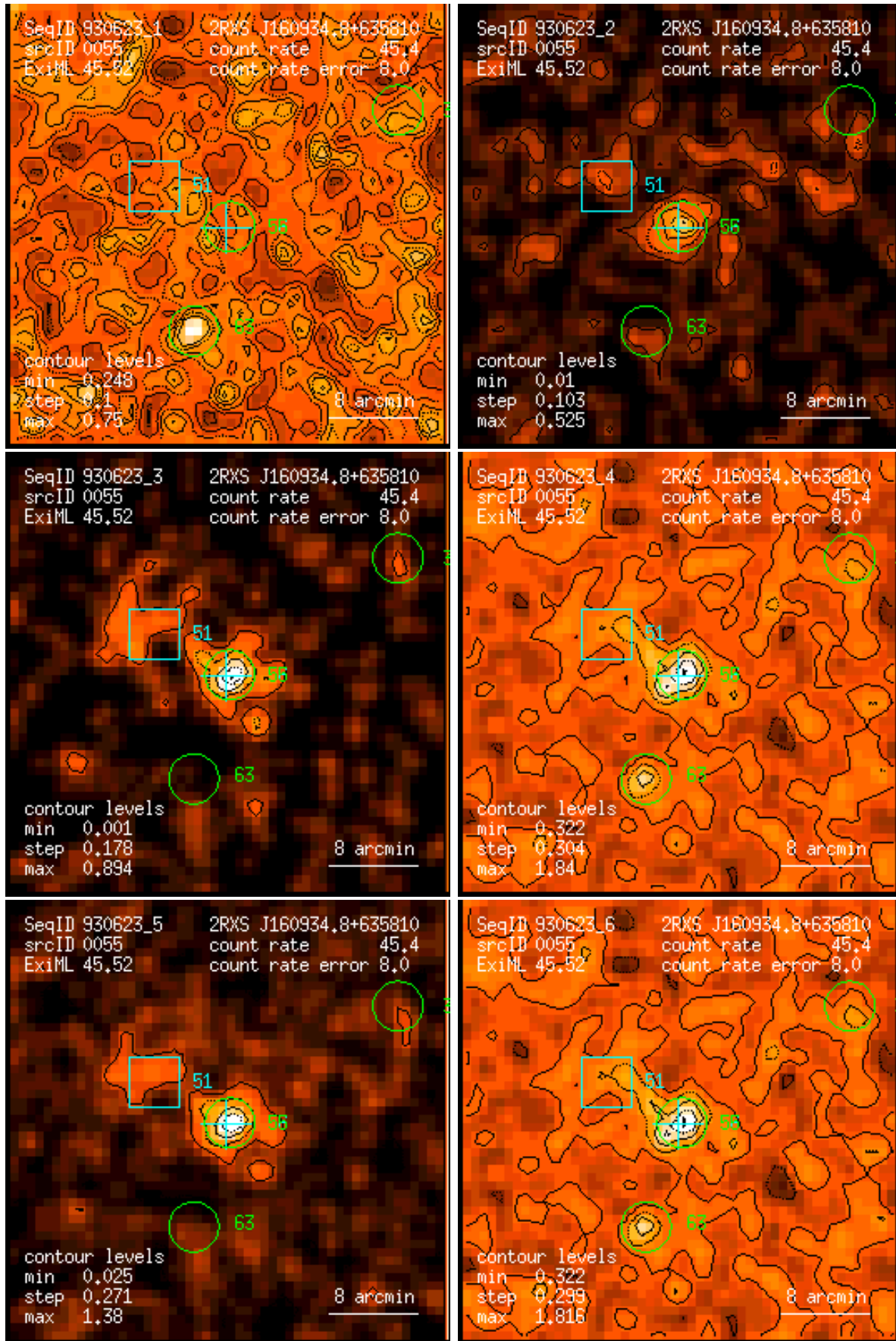
Figure 55: RASS 930623: detection 0055: band rate images, Gaussian filter: (1) PSPC channels 11 – 41, (2) 52 – 90, (3) 91 – 201, (4) 11 – 235, (5) 52 – 201, (6) 11 – 201. Broad band rates in counts/ks. Band rate contour levels in counts/ks/arcmin 2 .
