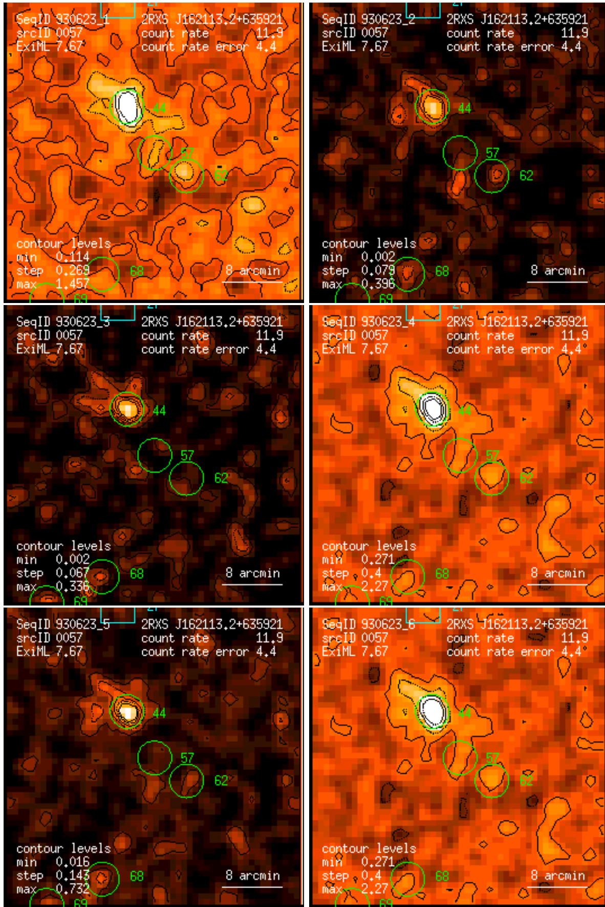
Figure 57: RASS 930623: detection 0057: band rate images, Gaussian filter: (1) PSPC channels 11 – 41, (2) 52 – 90, (3) 91 – 201, (4) 11 – 235, (5) 52 – 201, (6) 11 – 201. Broad band rates in counts/ks. Band rate contour levels in counts/ks/arcmin 2 .
