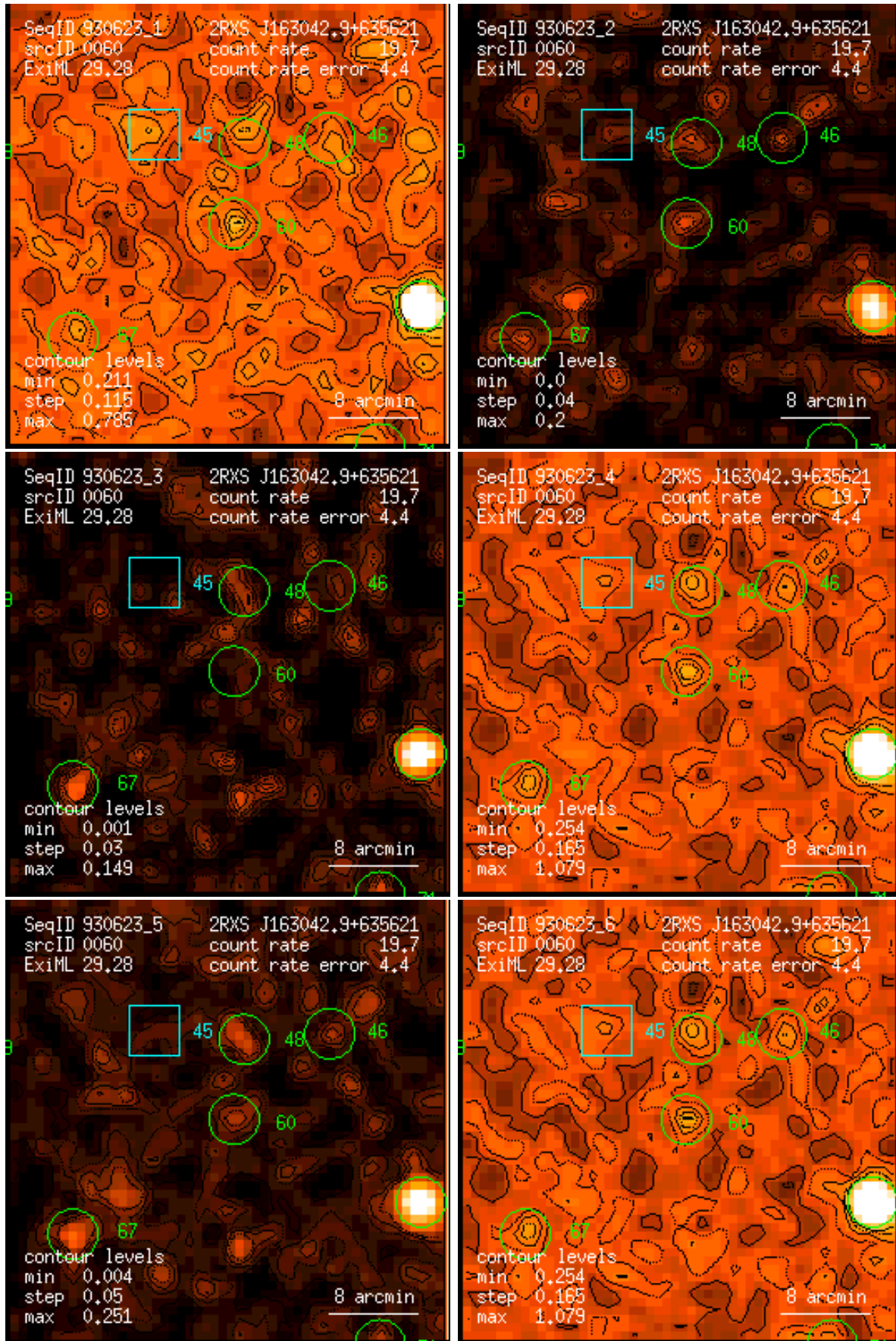
Figure 60: RASS 930623: detection 0060: band rate images, Gaussian filter: (1) PSPC channels 11 – 41, (2) 52 – 90, (3) 91 – 201, (4) 11 – 235, (5) 52 – 201, (6) 11 – 201. Broad band rates in counts/ks. Band rate contour levels in counts/ks/arcmin 2 .
