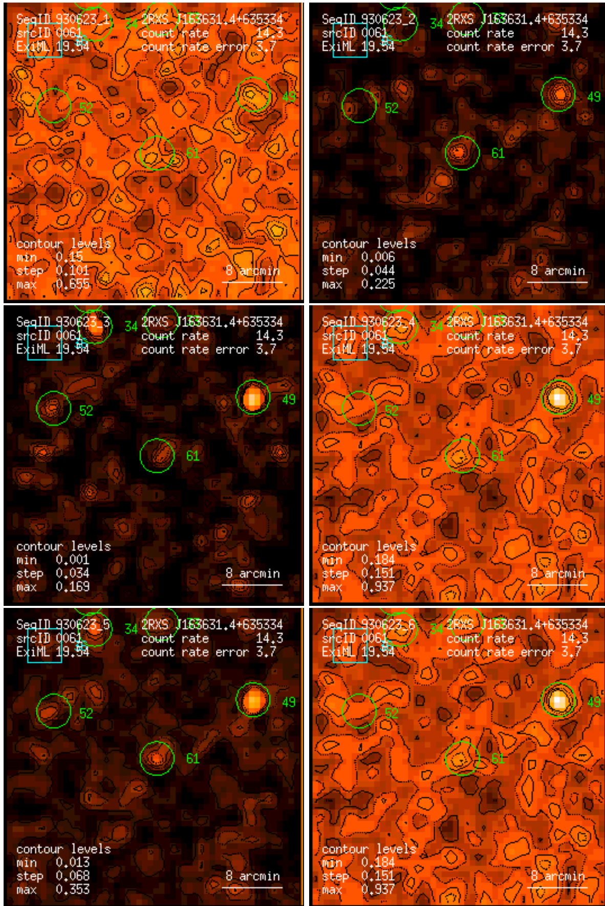
Figure 61: RASS 930623: detection 0061: band rate images, Gaussian filter: (1) PSPC channels 11 – 41, (2) 52 – 90, (3) 91 – 201, (4) 11 – 235, (5) 52 – 201, (6) 11 – 201. Broad band rates in counts/ks. Band rate contour levels in counts/ks/arcmin 2 .
