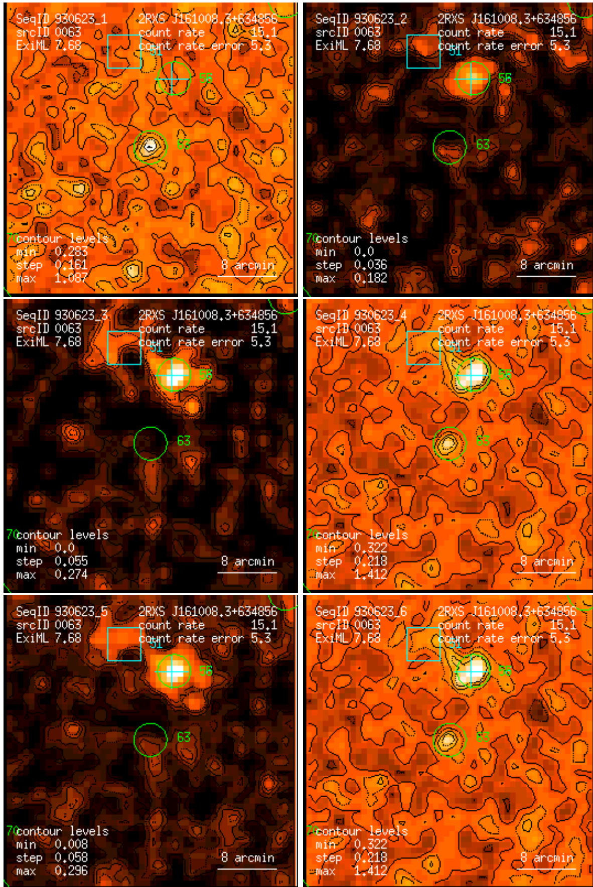
Figure 63: RASS 930623: detection 0063: band rate images, Gaussian filter: (1) PSPC channels 11 – 41, (2) 52 – 90, (3) 91 – 201, (4) 11 – 235, (5) 52 – 201, (6) 11 – 201. Broad band rates in counts/ks. Band rate contour levels in counts/ks/arcmin 2 .
