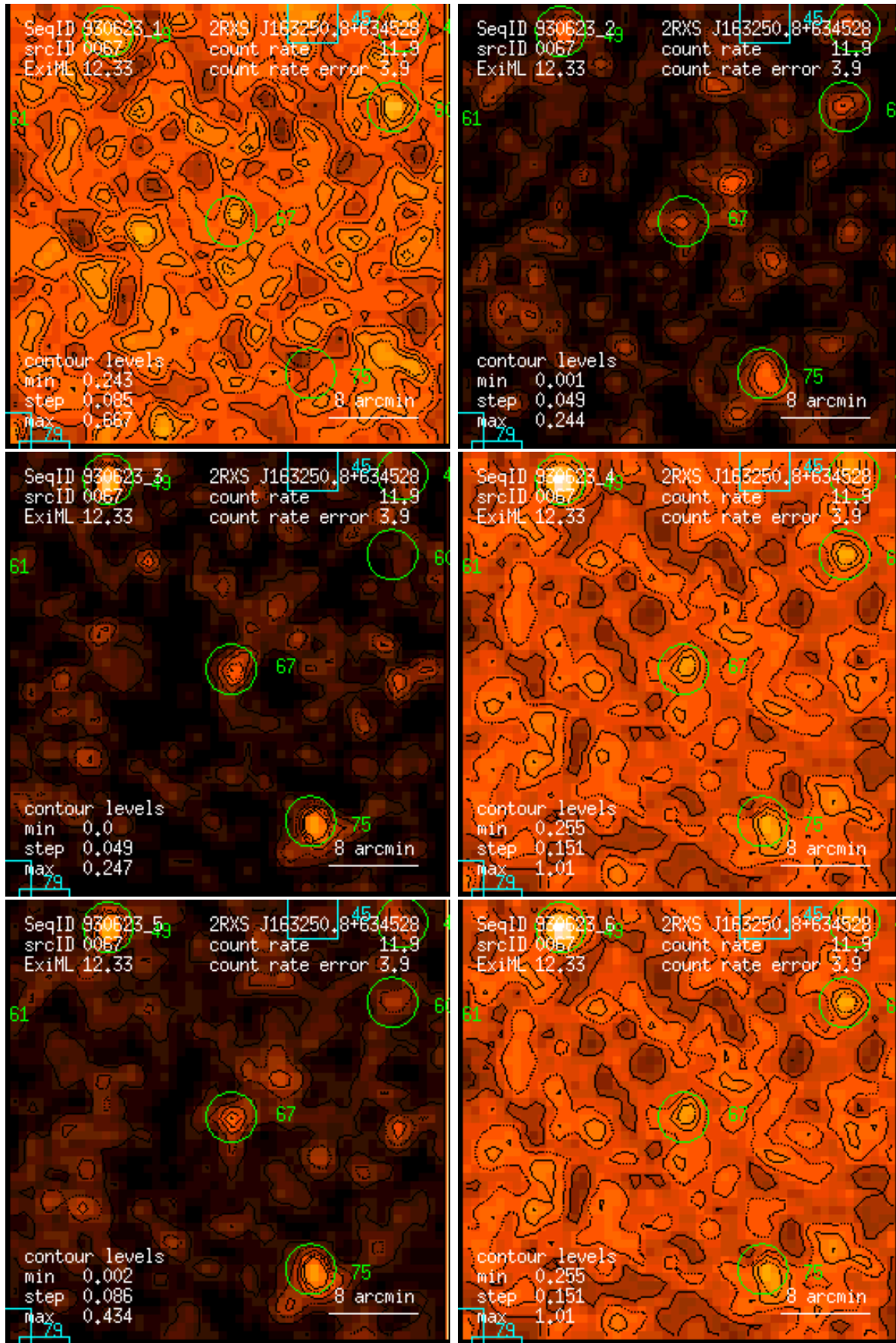
Figure 67: RASS 930623: detection 0067: band rate images, Gaussian filter: (1) PSPC channels 11 – 41, (2) 52 – 90, (3) 91 – 201, (4) 11 – 235, (5) 52 – 201, (6) 11 – 201. Broad band rates in counts/ks. Band rate contour levels in counts/ks/arcmin 2 .
