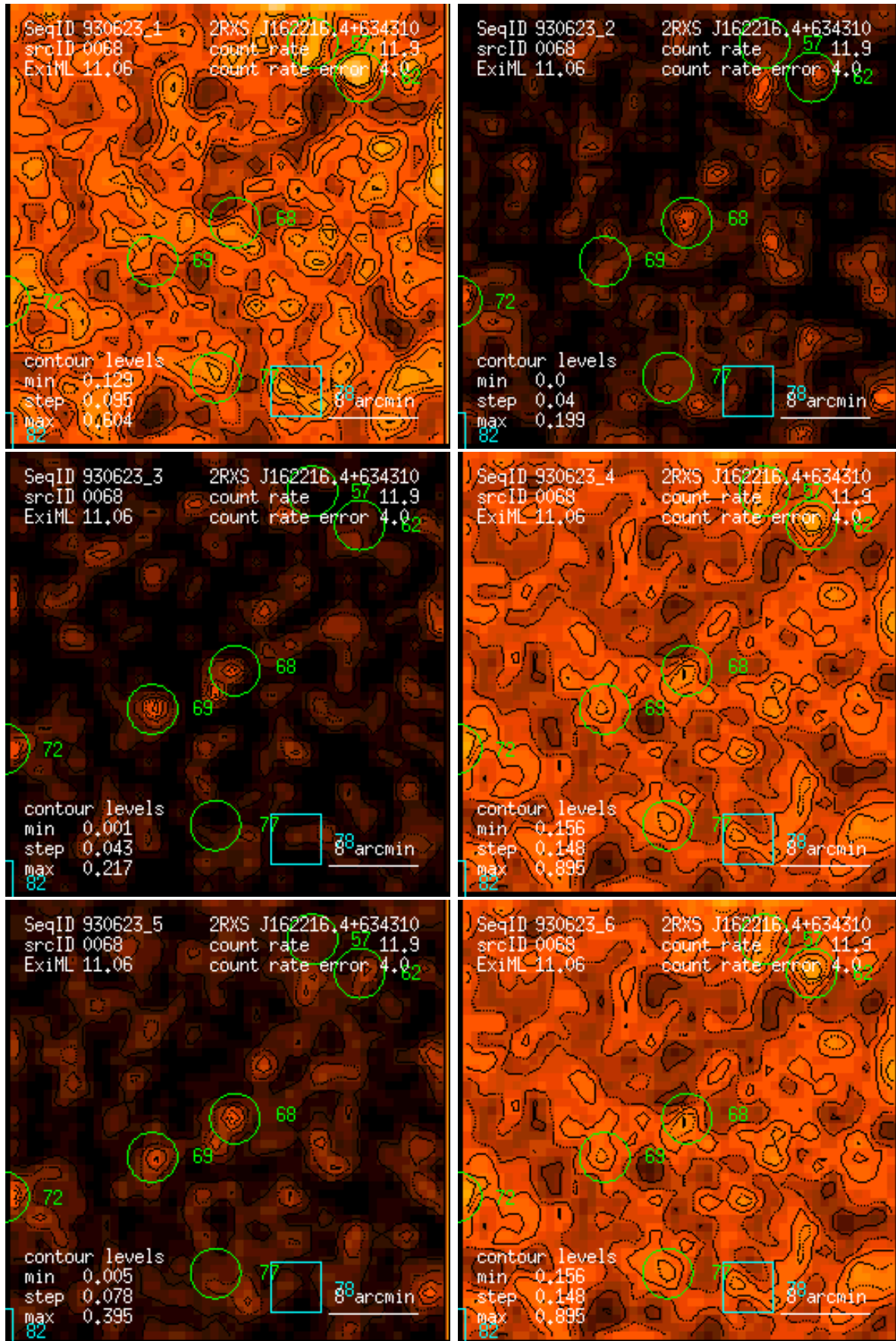
Figure 68: RASS 930623: detection 0068: band rate images, Gaussian filter: (1) PSPC channels 11 – 41, (2) 52 – 90, (3) 91 – 201, (4) 11 – 235, (5) 52 – 201, (6) 11 – 201. Broad band rates in counts/ks. Band rate contour levels in counts/ks/arcmin 2 .
