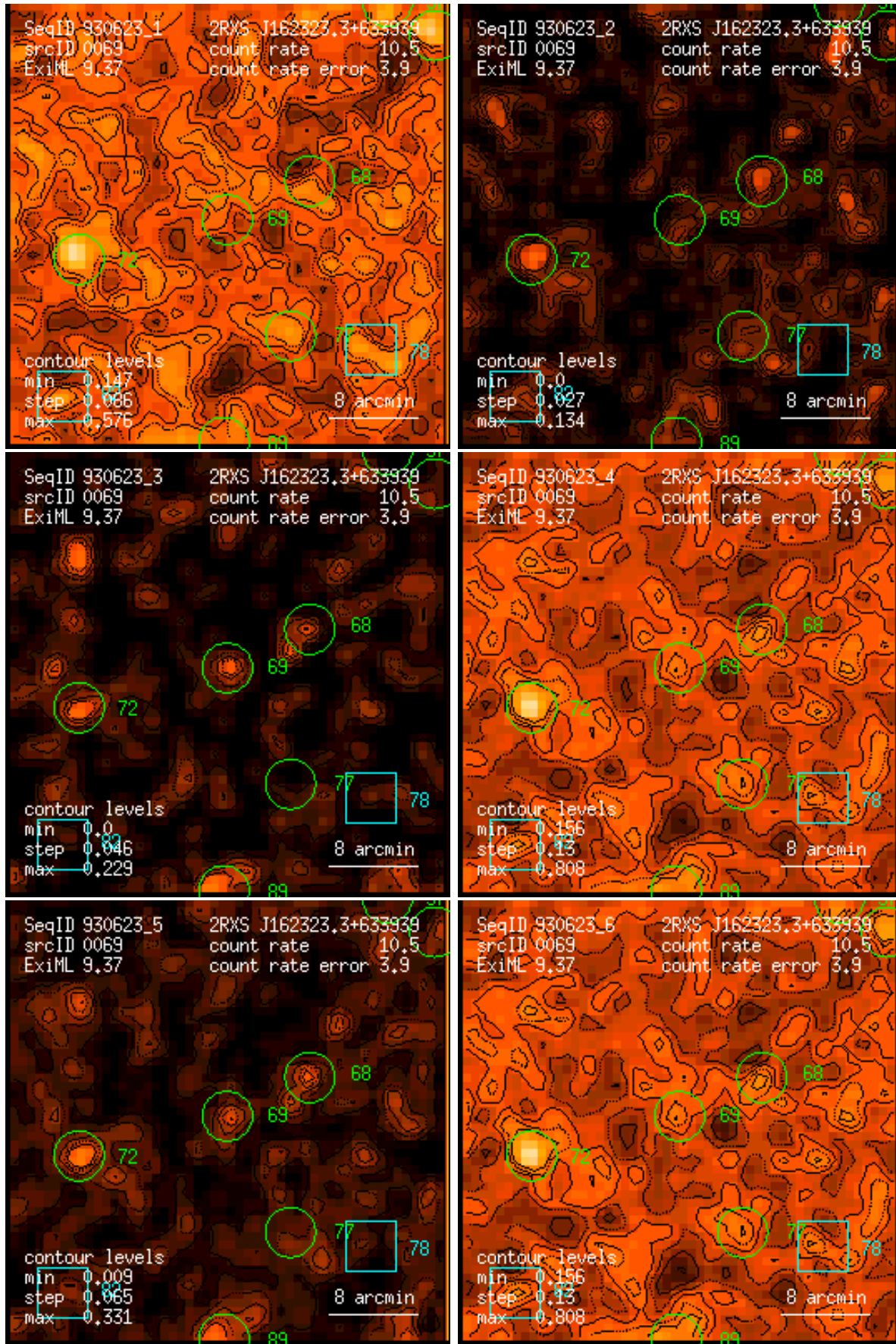
Figure 69: RASS 930623: detection 0069: band rate images, Gaussian filter: (1) PSPC channels 11 – 41, (2) 52 – 90, (3) 91 – 201, (4) 11 – 235, (5) 52 – 201, (6) 11 – 201. Broad band rates in counts/ks. Band rate contour levels in counts/ks/arcmin 2 .
