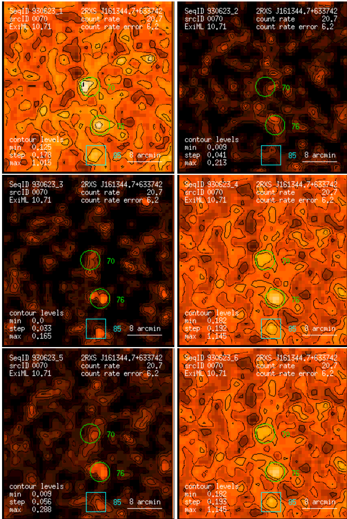
Figure 70: RASS 930623: detection 0070: band rate images, Gaussian filter: (1) PSPC channels 11 – 41, (2) 52 – 90, (3) 91 – 201, (4) 11 – 235, (5) 52 – 201, (6) 11 – 201. Broad band rates in counts/ks. Band rate contour levels in counts/ks/arcmin 2 .
