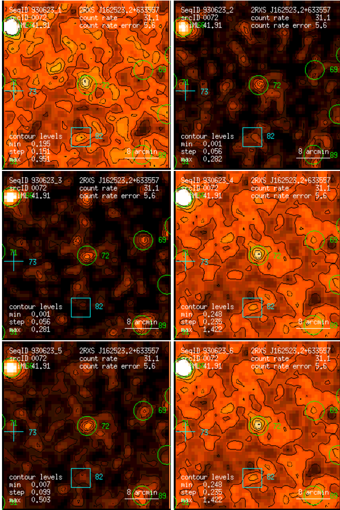
Figure 72: RASS 930623: detection 0072: band rate images, Gaussian filter: (1) PSPC channels 11 – 41, (2) 52 – 90, (3) 91 – 201, (4) 11 – 235, (5) 52 – 201, (6) 11 – 201. Broad band rates in counts/ks. Band rate contour levels in counts/ks/arcmin 2 .
