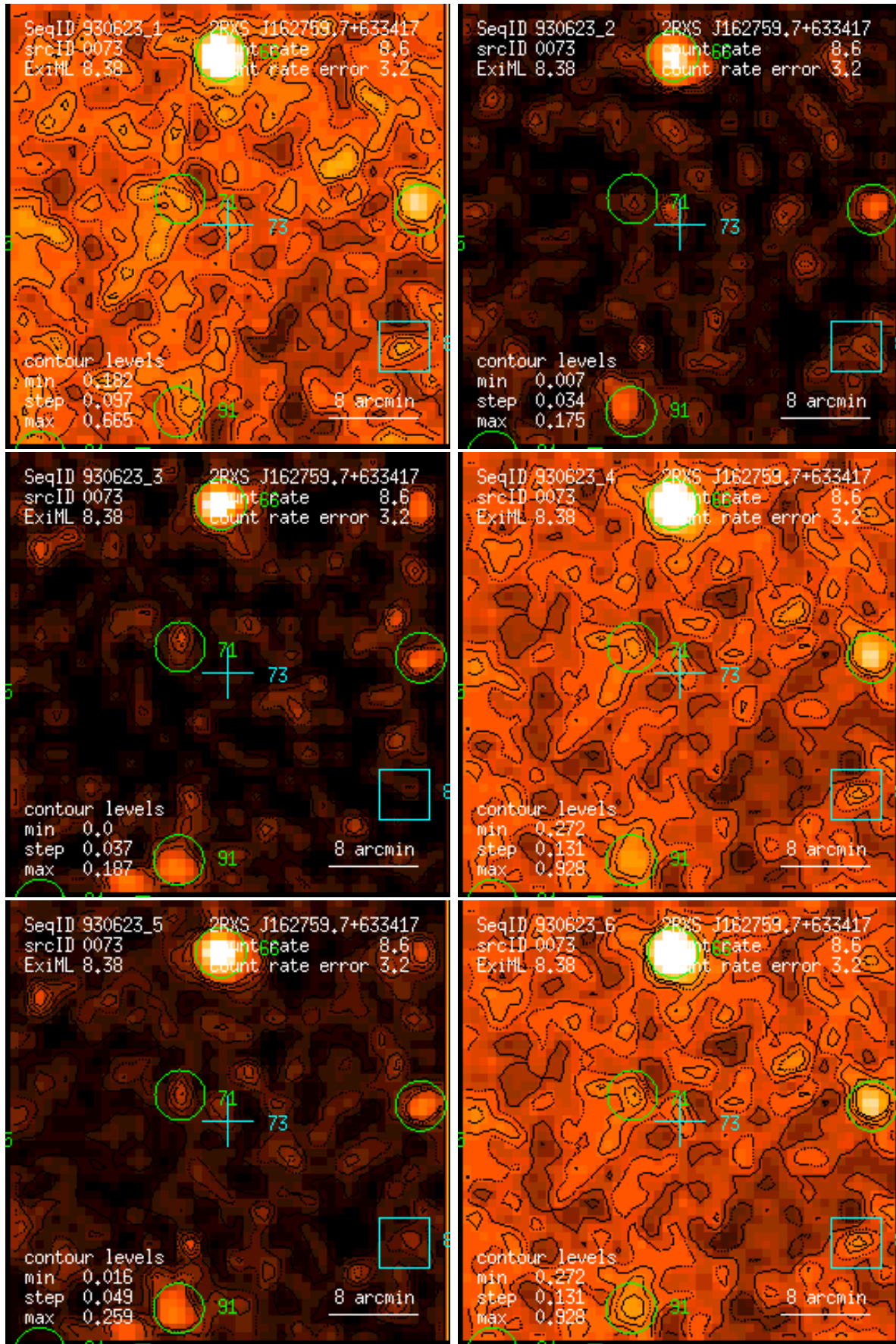
Figure 73: RASS 930623: detection 0073: band rate images, Gaussian filter: (1) PSPC channels 11 – 41, (2) 52 – 90, (3) 91 – 201, (4) 11 – 235, (5) 52 – 201, (6) 11 – 201. Broad band rates in counts/ks. Band rate contour levels in counts/ks/arcmin 2 .
