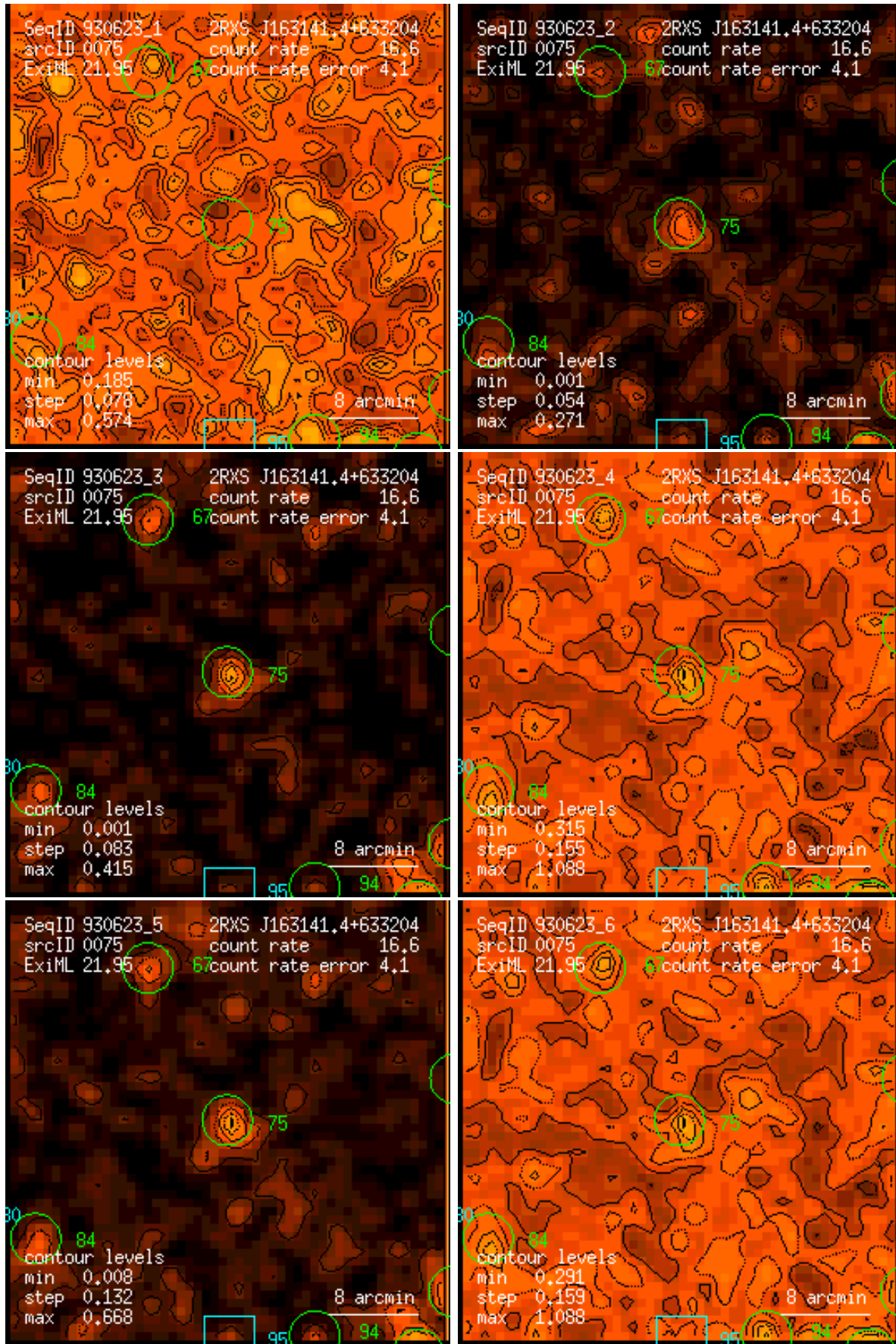
Figure 75: RASS 930623: detection 0075: band rate images, Gaussian filter: (1) PSPC channels 11 – 41, (2) 52 – 90, (3) 91 – 201, (4) 11 – 235, (5) 52 – 201, (6) 11 – 201. Broad band rates in counts/ks. Band rate contour levels in counts/ks/arcmin 2 .
