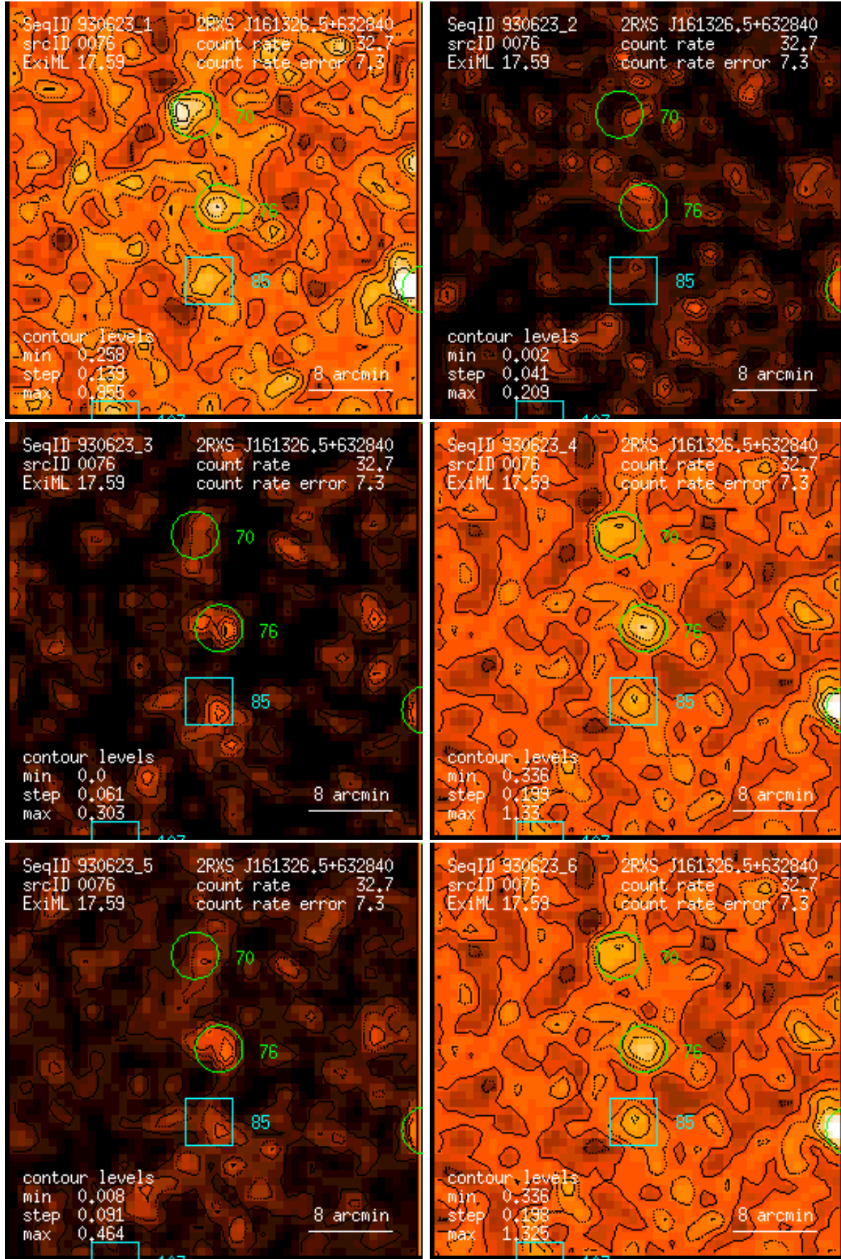
Figure 76: RASS 930623: detection 0076: band rate images, Gaussian filter: (1) PSPC channels 11 – 41, (2) 52 – 90, (3) 91 – 201, (4) 11 – 235, (5) 52 – 201, (6) 11 – 201. Broad band rates in counts/ks. Band rate contour levels in counts/ks/arcmin 2 .
