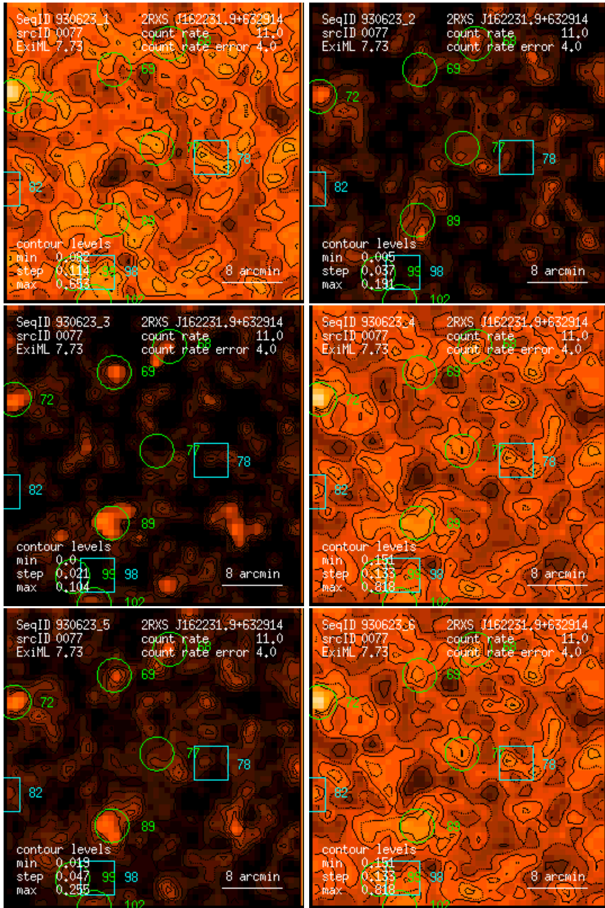
Figure 77: RASS 930623: detection 0077: band rate images, Gaussian filter: (1) PSPC channels 11 – 41, (2) 52 – 90, (3) 91 – 201, (4) 11 – 235, (5) 52 – 201, (6) 11 – 201. Broad band rates in counts/ks. Band rate contour levels in counts/ks/arcmin 2 .
