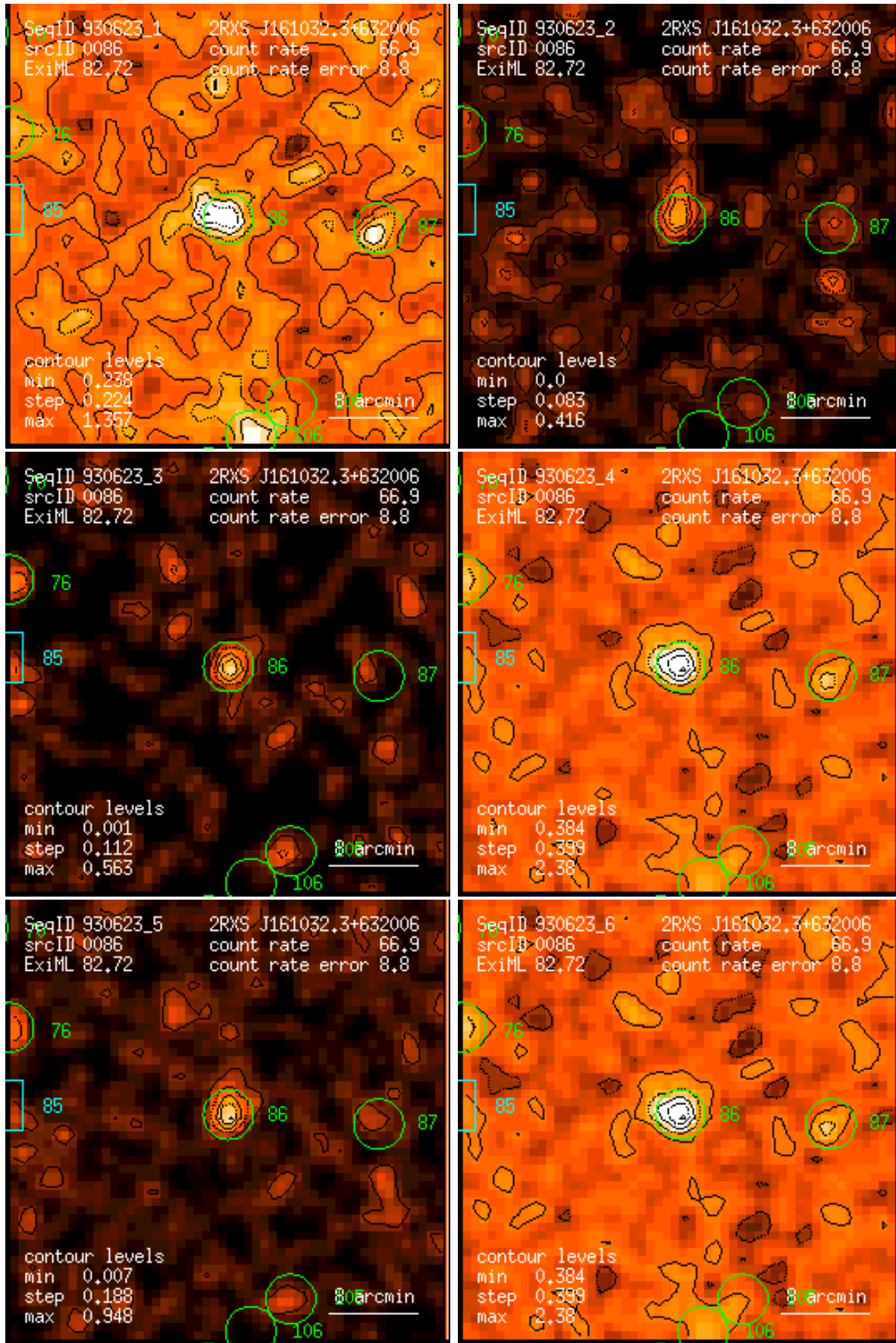
Figure 86: RASS 930623: detection 0086: band rate images, Gaussian filter: (1) PSPC channels 11 – 41, (2) 52 – 90, (3) 91 – 201, (4) 11 – 235, (5) 52 – 201, (6) 11 – 201. Broad band rates in counts/ks. Band rate contour levels in counts/ks/arcmin 2 .
