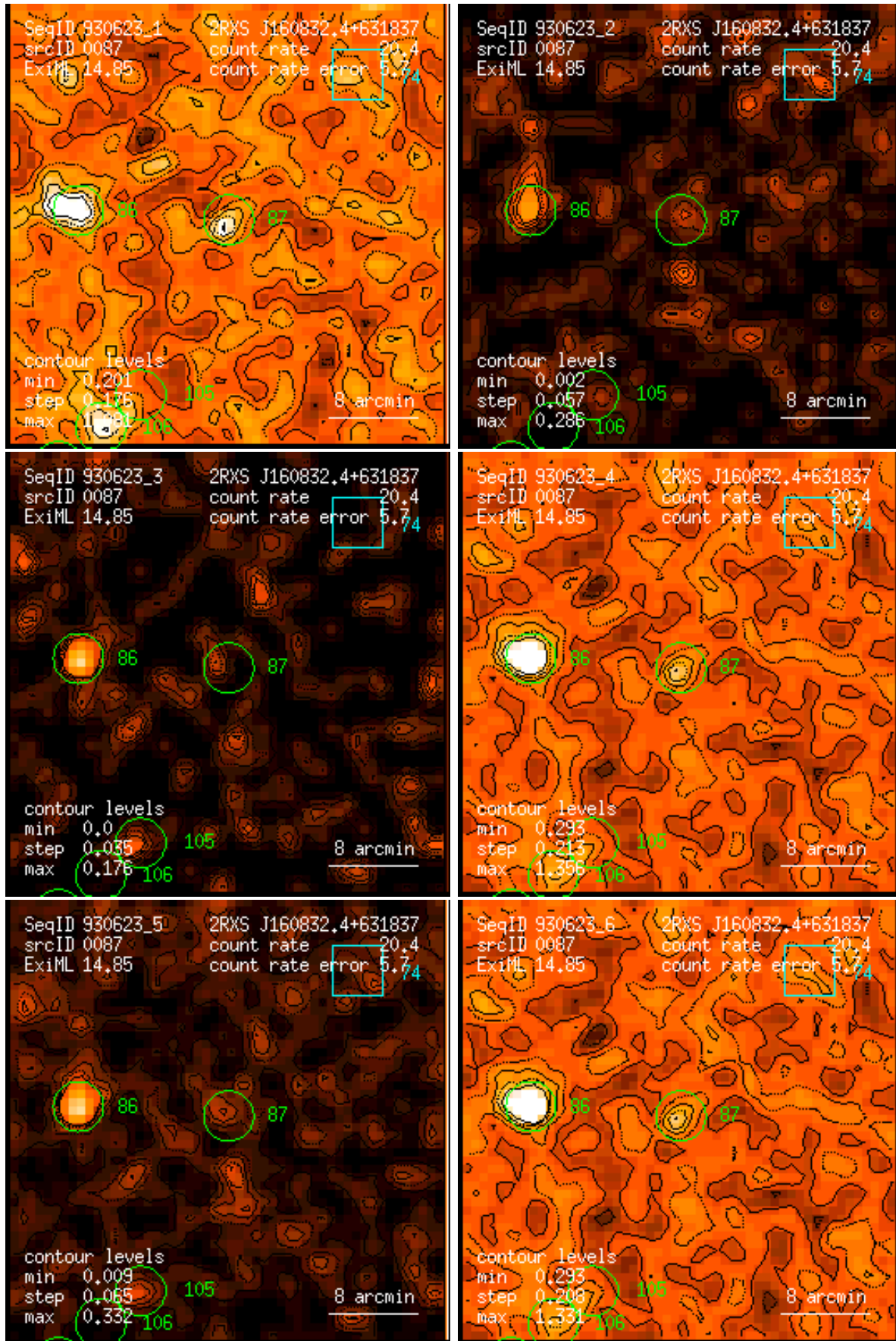
Figure 87: RASS 930623: detection 0087: band rate images, Gaussian filter: (1) PSPC channels 11 – 41, (2) 52 – 90, (3) 91 – 201, (4) 11 – 235, (5) 52 – 201, (6) 11 – 201. Broad band rates in counts/ks. Band rate contour levels in counts/ks/arcmin 2 .
