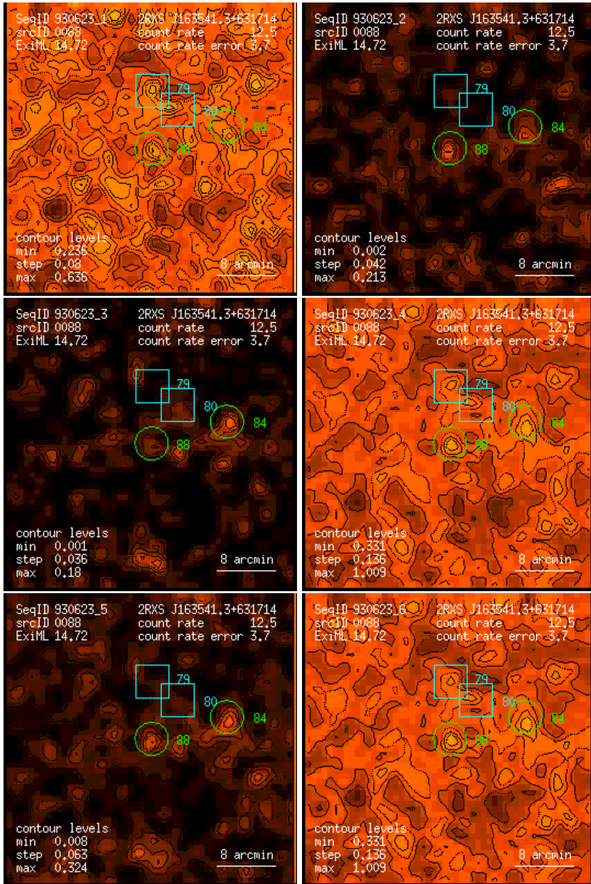
Figure 88: RASS 930623: detection 0088: band rate images, Gaussian filter: (1) PSPC channels 11 – 41, (2) 52 – 90, (3) 91 – 201, (4) 11 – 235, (5) 52 – 201, (6) 11 – 201. Broad band rates in counts/ks. Band rate contour levels in counts/ks/arcmin 2 .
