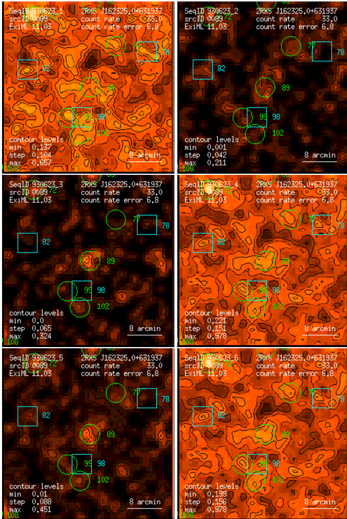
Figure 89: RASS 930623: detection 0089: band rate images, Gaussian filter: (1) PSPC channels 11 – 41, (2) 52 – 90, (3) 91 – 201, (4) 11 – 235, (5) 52 – 201, (6) 11 – 201. Broad band rates in counts/ks. Band rate contour levels in counts/ks/arcmin 2 .
