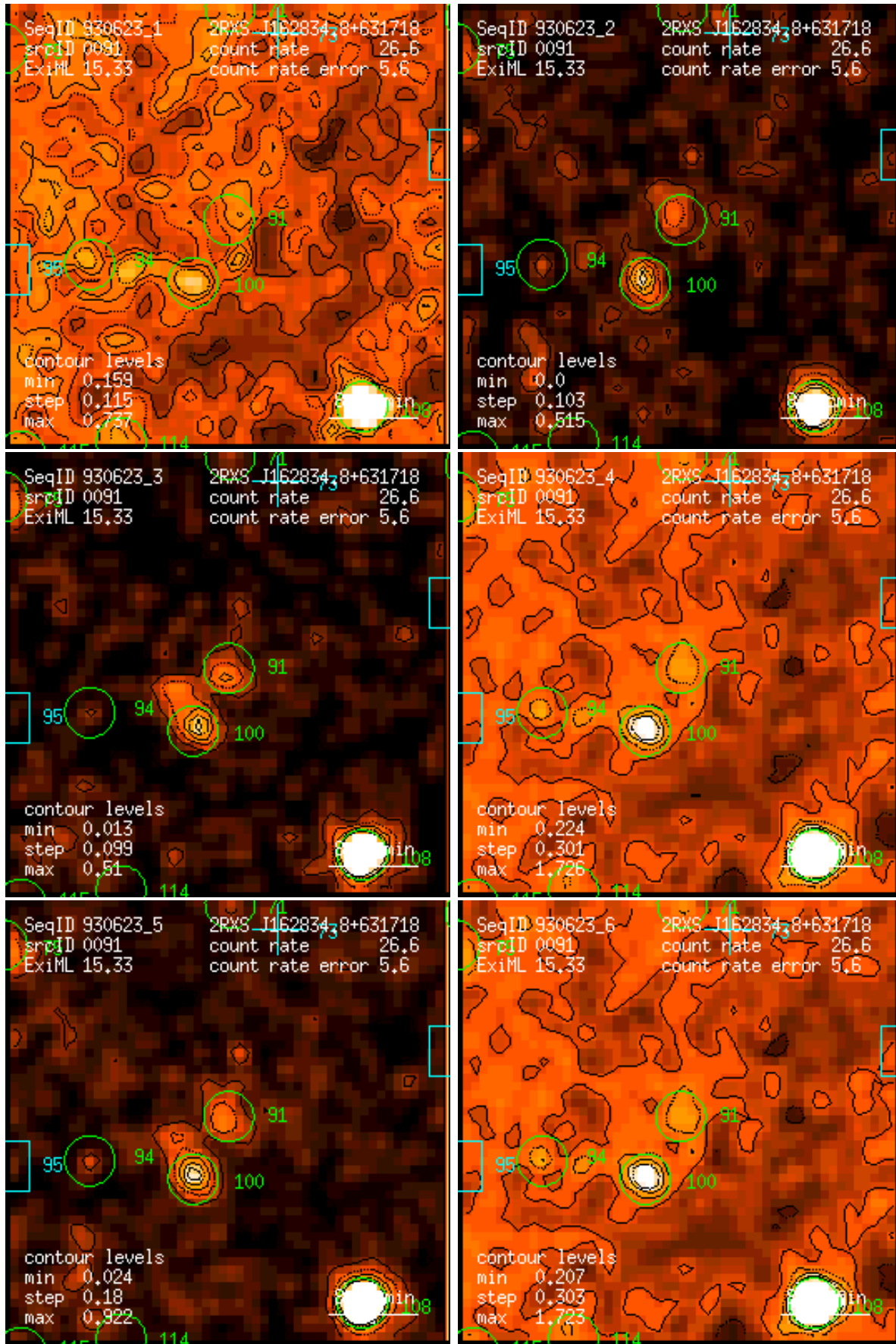
Figure 91: RASS 930623: detection 0091: band rate images, Gaussian filter: (1) PSPC channels 11 – 41, (2) 52 – 90, (3) 91 – 201, (4) 11 – 235, (5) 52 – 201, (6) 11 – 201. Broad band rates in counts/ks. Band rate contour levels in counts/ks/arcmin 2 .
