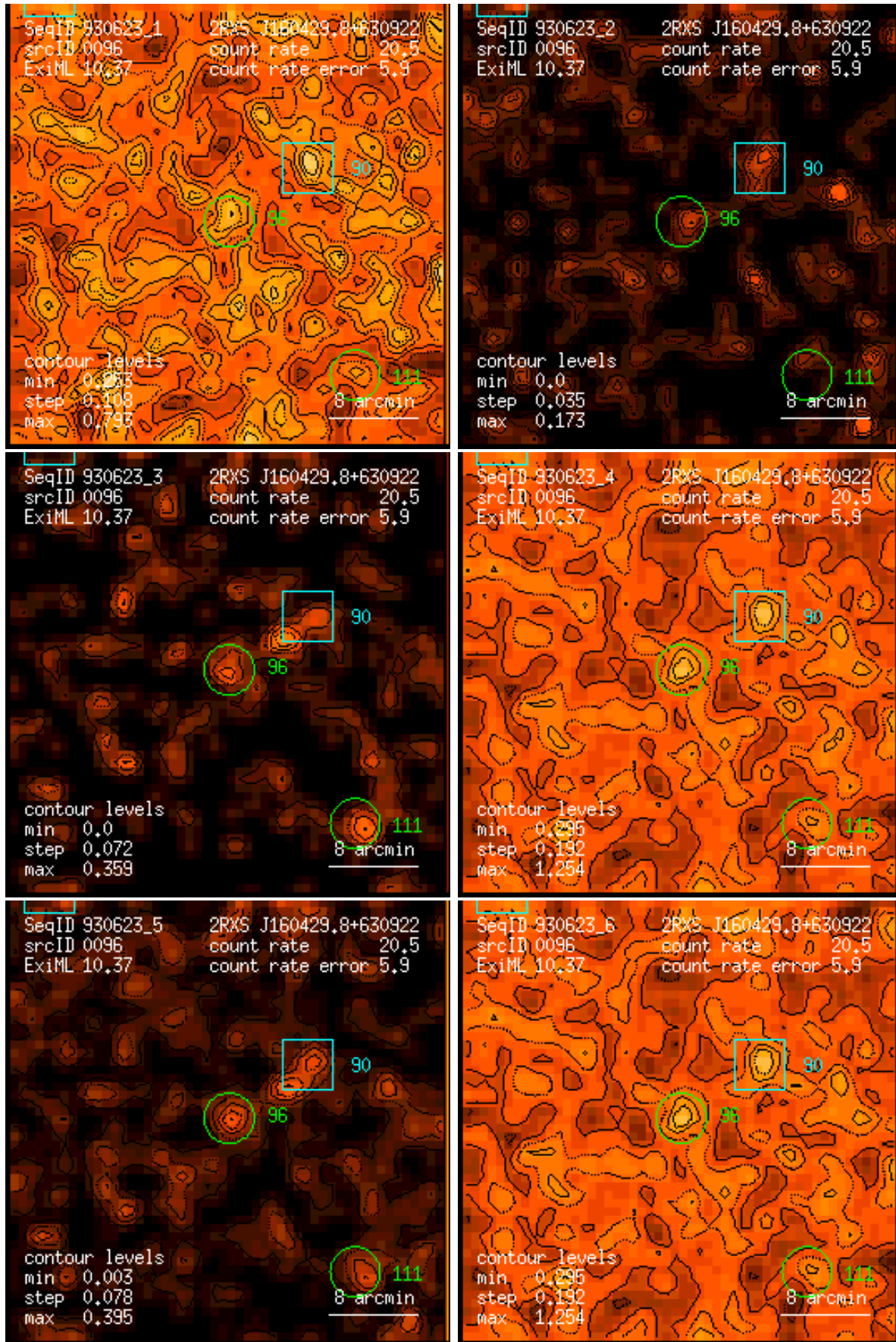
Figure 96: RASS 930623: detection 0096: band rate images, Gaussian filter: (1) PSPC channels 11 – 41, (2) 52 – 90, (3) 91 – 201, (4) 11 – 235, (5) 52 – 201, (6) 11 – 201. Broad band rates in counts/ks. Band rate contour levels in counts/ks/arcmin 2 .
